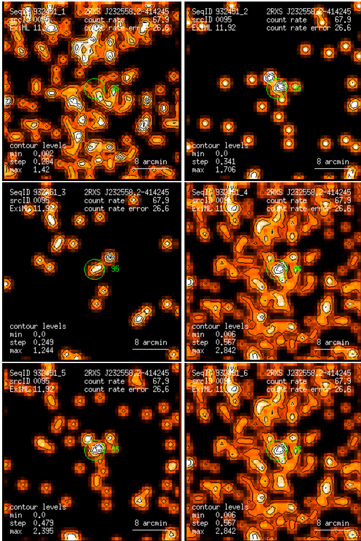
Figure 95: RASS 932451: detection 0095: band rate images, Gaussian filter: (1) PSPC channels 11 – 41, (2) 52 – 90, (3) 91 – 201, (4) 11 – 235, (5) 52 – 201, (6) 11 – 201. Broad band rates in counts/ks. Band rate contour levels in counts/ks/arcmin 2 .
