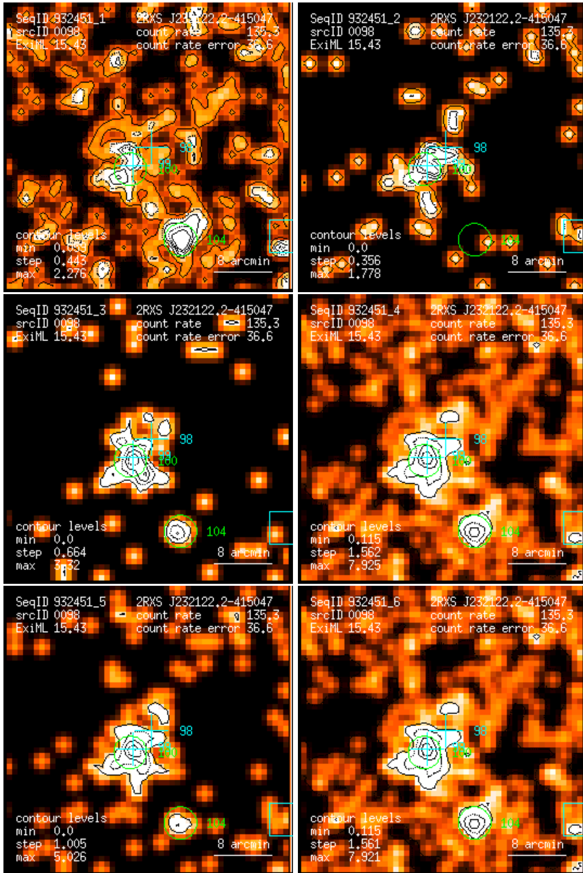
Figure 98: RASS 932451: detection 0098: band rate images, Gaussian filter: (1) PSPC channels 11 – 41, (2) 52 – 90, (3) 91 – 201, (4) 11 – 235, (5) 52 – 201, (6) 11 – 201. Broad band rates in counts/ks. Band rate contour levels in counts/ks/arcmin 2 .
