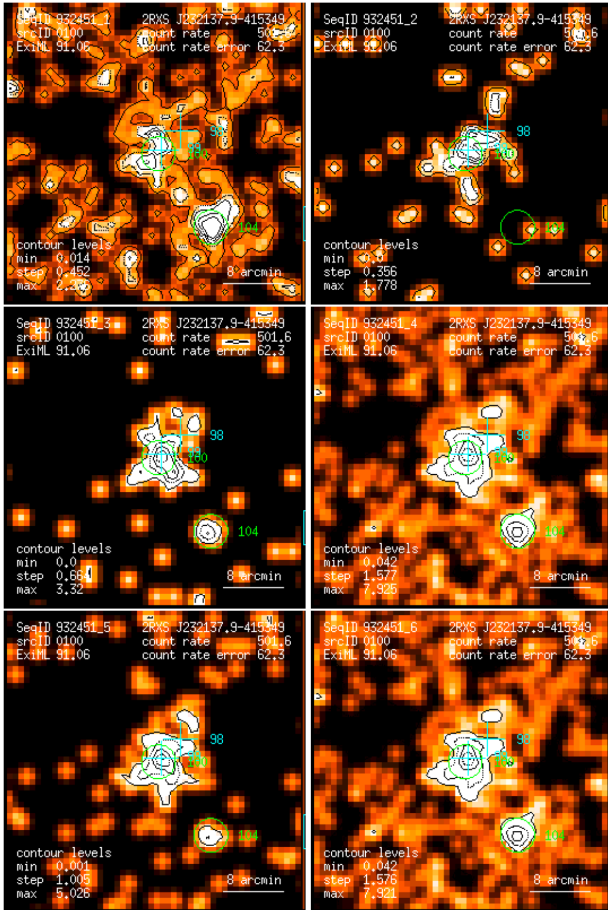
Figure 100: RASS 932451: detection 0100: band rate images, Gaussian filter: (1) PSPC channels 11 – 41, (2) 52 – 90, (3) 91 – 201, (4) 11 – 235, (5) 52 – 201, (6) 11 – 201. Broad band rates in counts/ks. Band rate contour levels in counts/ks/arcmin 2 .
