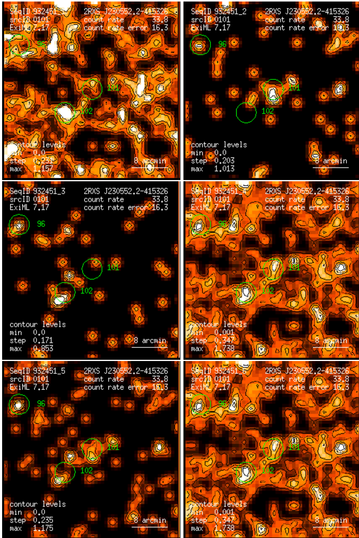
Figure 101: RASS 932451: detection 0101: band rate images, Gaussian filter: (1) PSPC channels 11 – 41, (2) 52 – 90, (3) 91 – 201, (4) 11 – 235, (5) 52 – 201, (6) 11 – 201. Broad band rates in counts/ks. Band rate contour levels in counts/ks/arcmin 2 .
