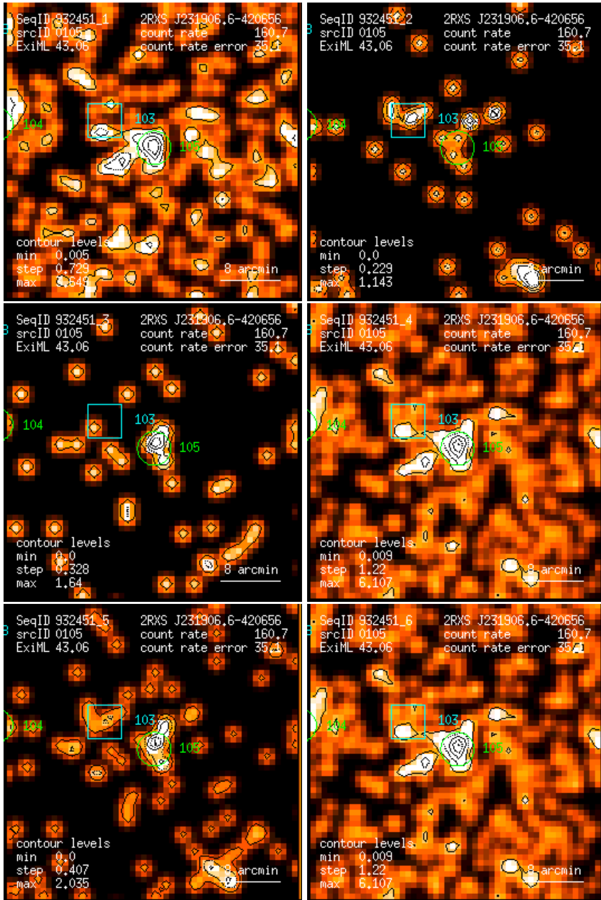
Figure 105: RASS 932451: detection 0105: band rate images, Gaussian filter: (1) PSPC channels 11 – 41, (2) 52 – 90, (3) 91 – 201, (4) 11 – 235, (5) 52 – 201, (6) 11 – 201. Broad band rates in counts/ks. Band rate contour levels in counts/ks/arcmin 2 .
