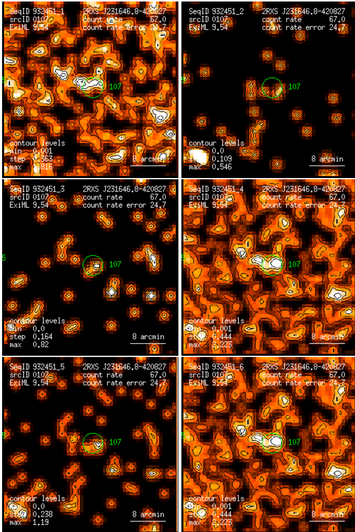
Figure 107: RASS 932451: detection 0107: band rate images, Gaussian filter: (1) PSPC channels 11 – 41, (2) 52 – 90, (3) 91 – 201, (4) 11 – 235, (5) 52 – 201, (6) 11 – 201. Broad band rates in counts/ks. Band rate contour levels in counts/ks/arcmin 2 .
