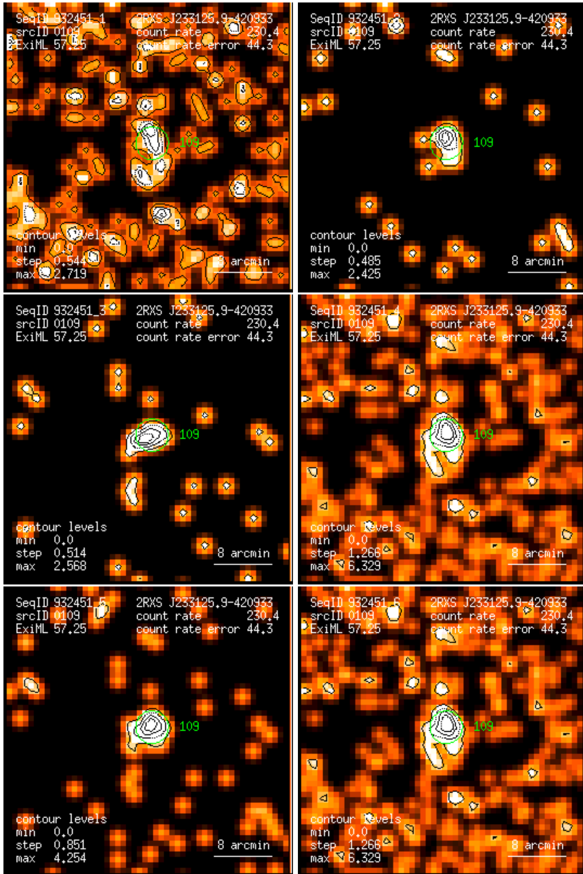
Figure 109: RASS 932451: detection 0109: band rate images, Gaussian filter: (1) PSPC channels 11 – 41, (2) 52 – 90, (3) 91 – 201, (4) 11 – 235, (5) 52 – 201, (6) 11 – 201. Broad band rates in counts/ks. Band rate contour levels in counts/ks/arcmin 2 .
