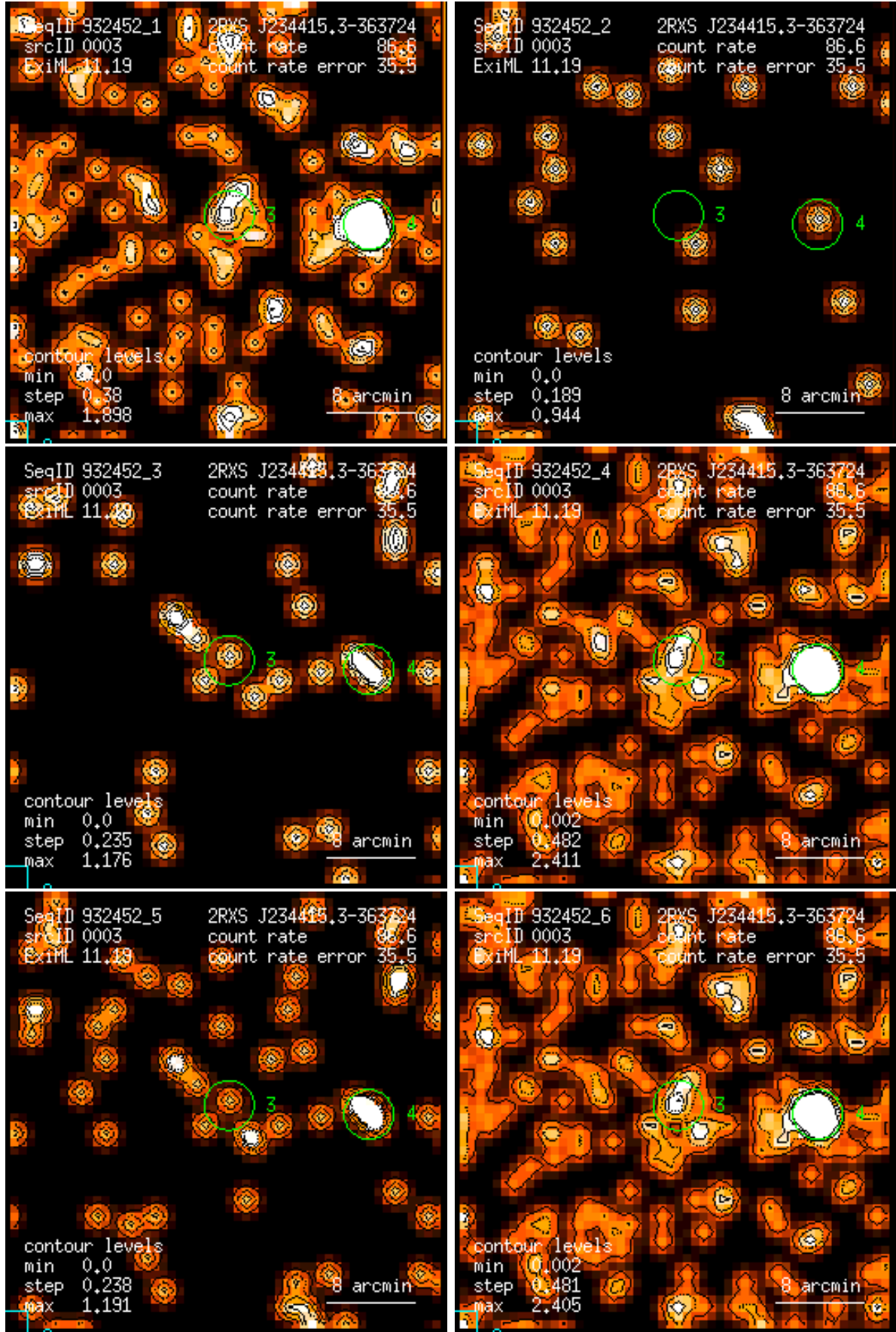
Figure 3: RASS 932452: detection 0003: band rate images, Gaussian filter: (1) PSPC channels 11 – 41, (2) 52 – 90, (3) 91 – 201, (4) 11 – 235, (5) 52 – 201, (6) 11 – 201. Broad band rates in counts/ks. Band rate contour levels in counts/ks/arcmin 2 .
