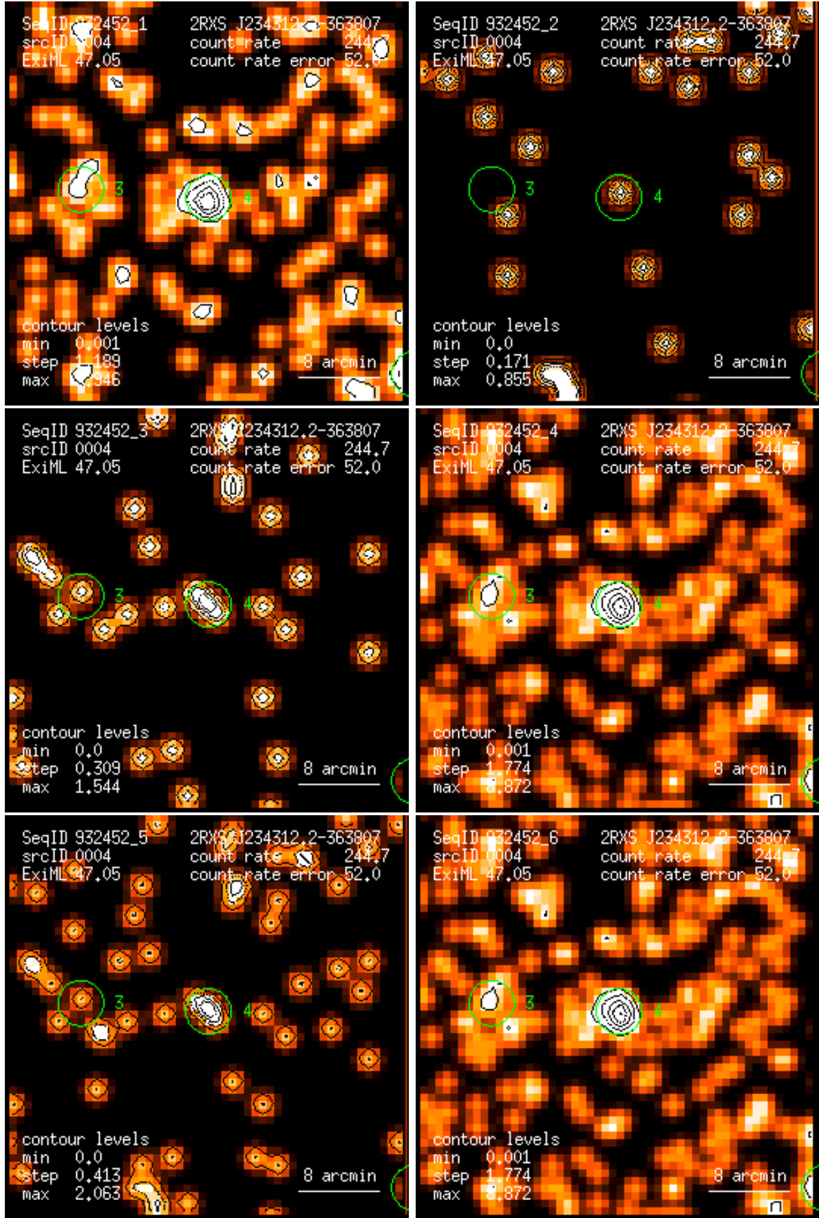
Figure 4: RASS 932452: detection 0004: band rate images, Gaussian filter: (1) PSPC channels 11 – 41, (2) 52 – 90, (3) 91 – 201, (4) 11 – 235, (5) 52 – 201, (6) 11 – 201. Broad band rates in counts/ks. Band rate contour levels in counts/ks/arcmin 2 .
