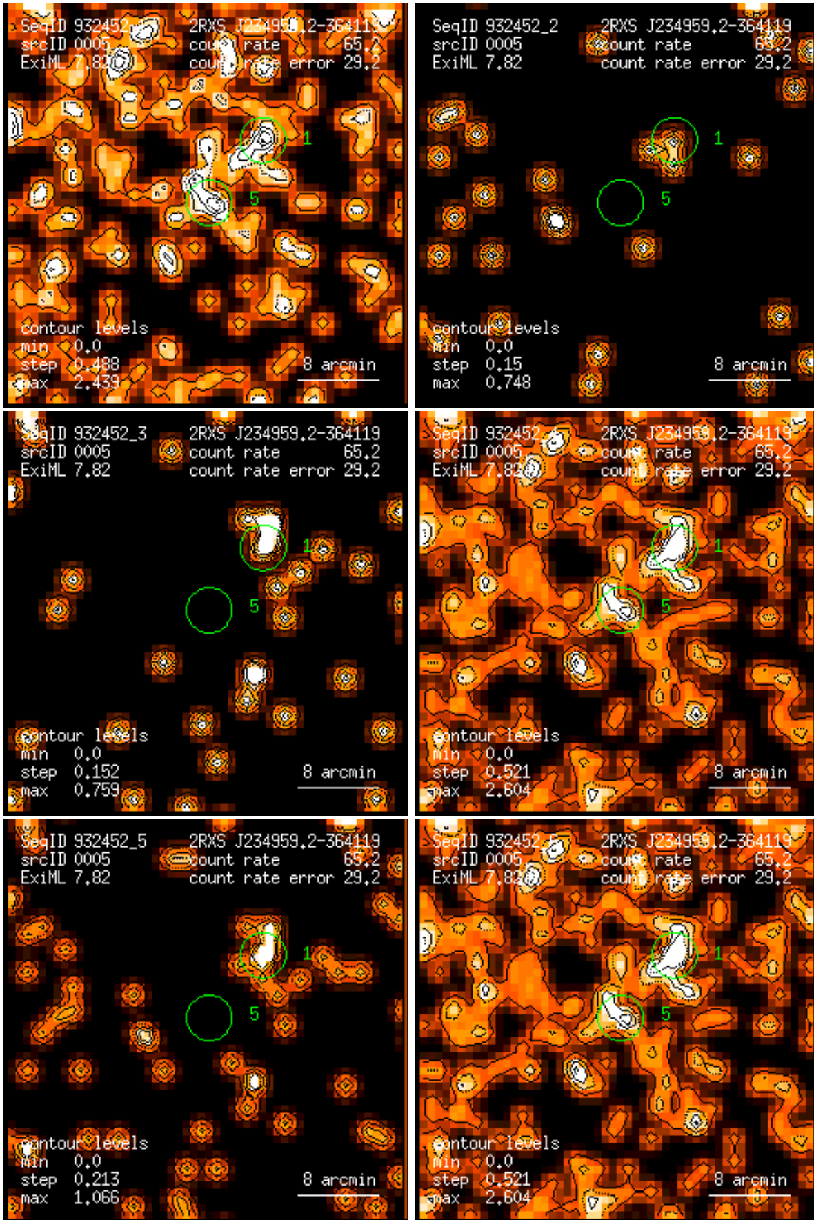
Figure 5: RASS 932452: detection 0005: band rate images, Gaussian filter: (1) PSPC channels 11 – 41, (2) 52 – 90, (3) 91 – 201, (4) 11 – 235, (5) 52 – 201, (6) 11 – 201. Broad band rates in counts/ks. Band rate contour levels in counts/ks/arcmin 2 .
