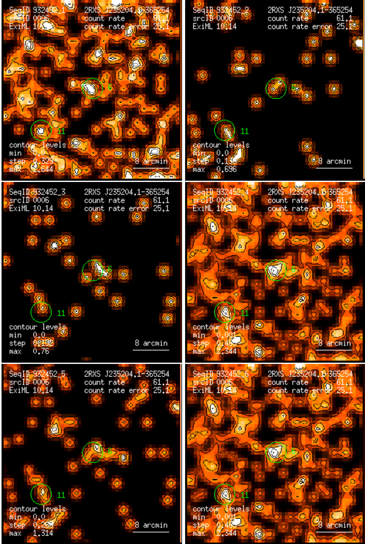
Figure 6: RASS 932452: detection 0006: band rate images, Gaussian filter: (1) PSPC channels 11 – 41, (2) 52 – 90, (3) 91 – 201, (4) 11 – 235, (5) 52 – 201, (6) 11 – 201. Broad band rates in counts/ks. Band rate contour levels in counts/ks/arcmin 2 .
