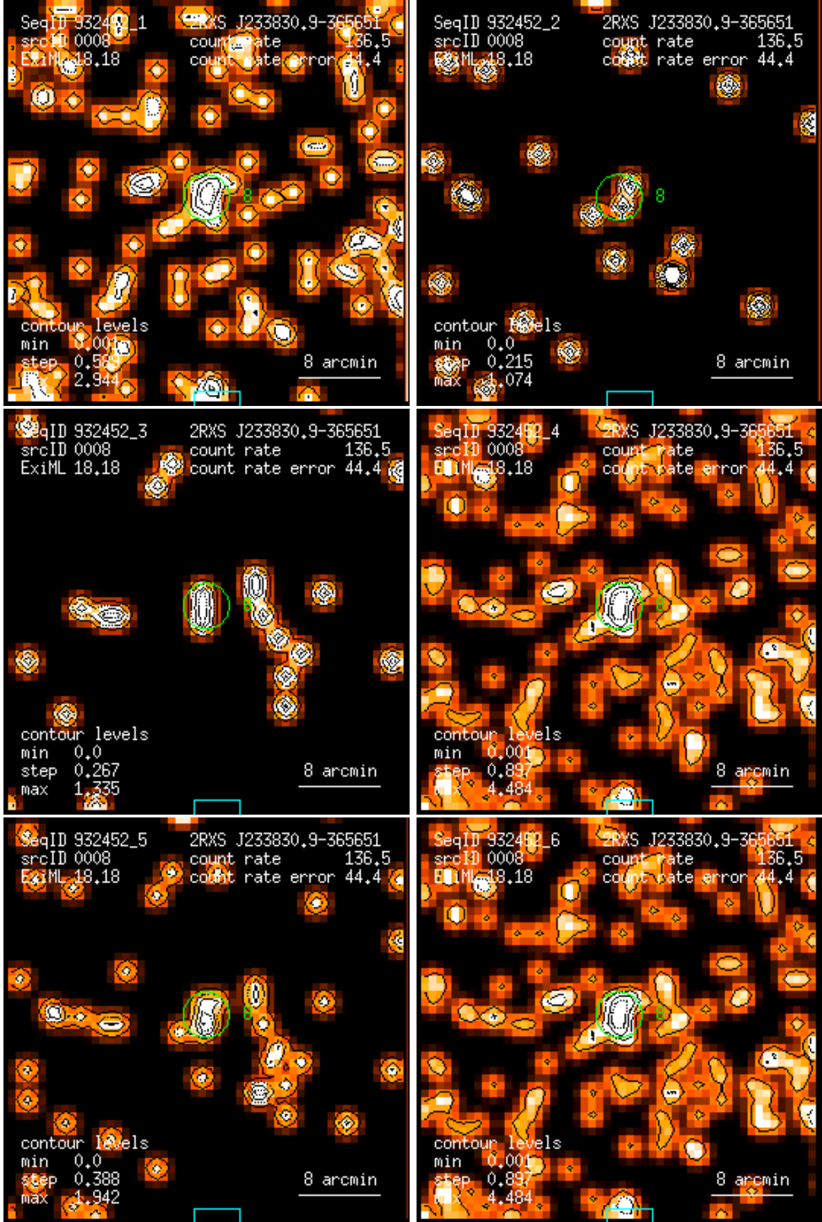
Figure 8: RASS 932452: detection 0008: band rate images, Gaussian filter: (1) PSPC channels 11 – 41, (2) 52 – 90, (3) 91 – 201, (4) 11 – 235, (5) 52 – 201, (6) 11 – 201. Broad band rates in counts/ks. Band rate contour levels in counts/ks/arcmin 2 .
