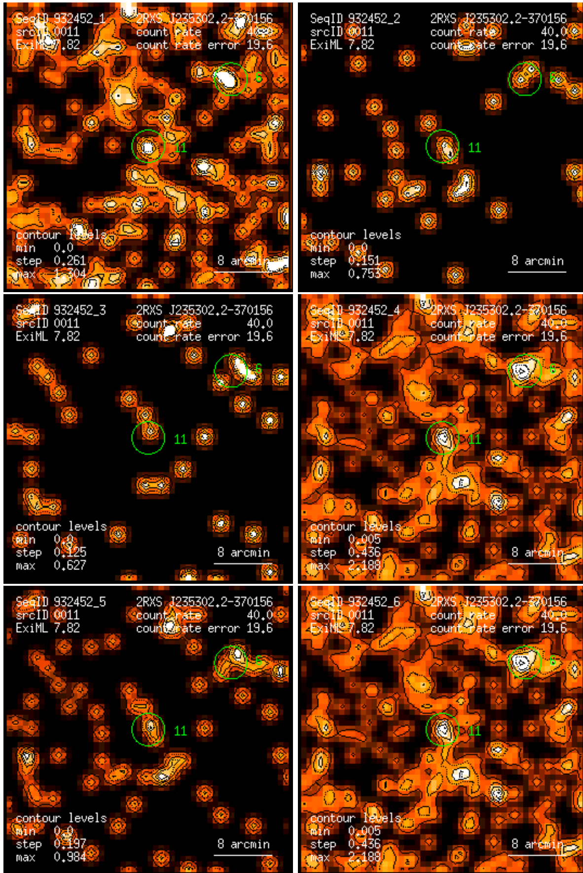
Figure 11: RASS 932452: detection 0011: band rate images, Gaussian filter: (1) PSPC channels 11 – 41, (2) 52 – 90, (3) 91 – 201, (4) 11 – 235, (5) 52 – 201, (6) 11 – 201. Broad band rates in counts/ks. Band rate contour levels in counts/ks/arcmin 2 .
