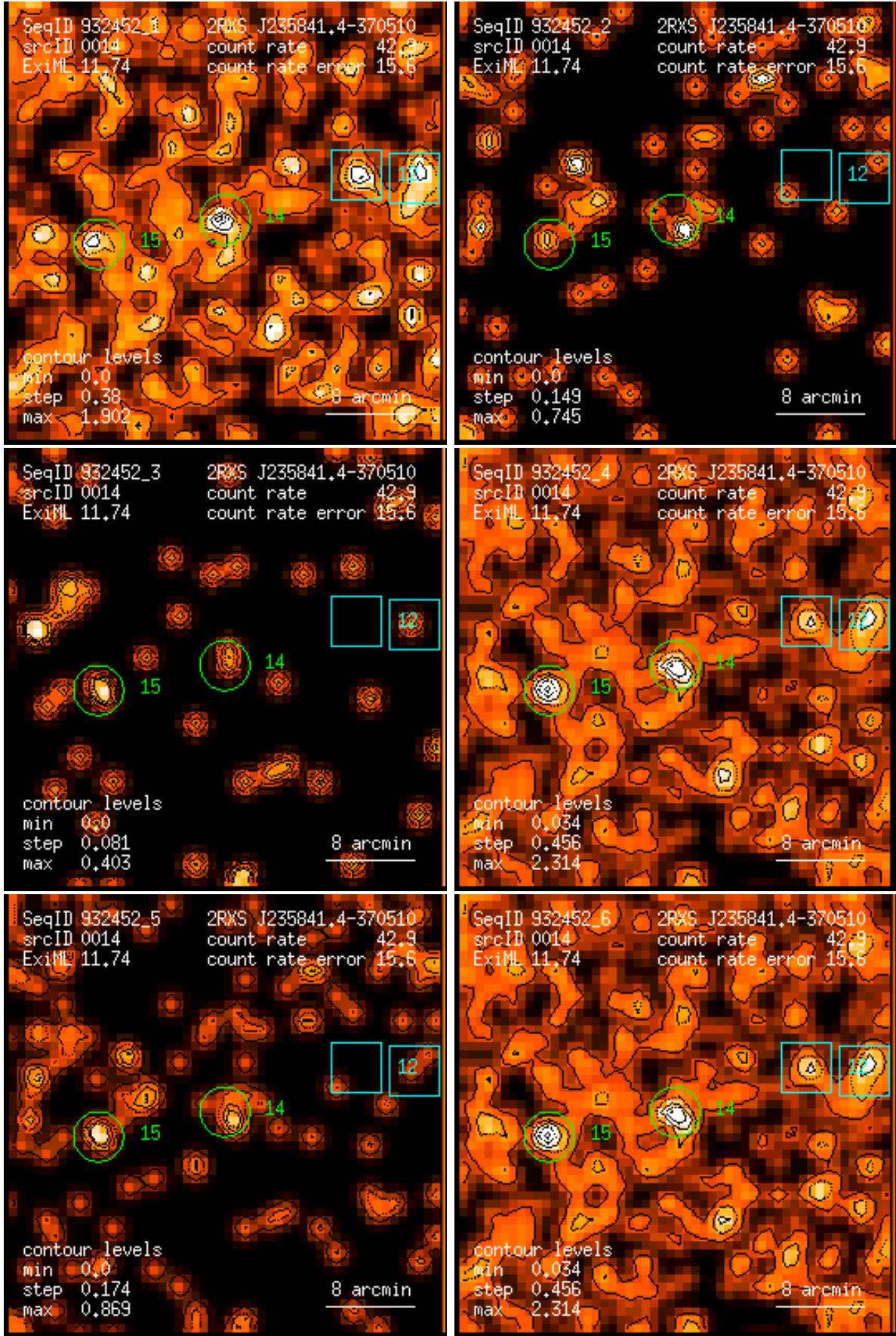
Figure 14: RASS 932452: detection 0014: band rate images, Gaussian filter: (1) PSPC channels 11 – 41, (2) 52 – 90, (3) 91 – 201, (4) 11 – 235, (5) 52 – 201, (6) 11 – 201. Broad band rates in counts/ks. Band rate contour levels in counts/ks/arcmin 2 .
