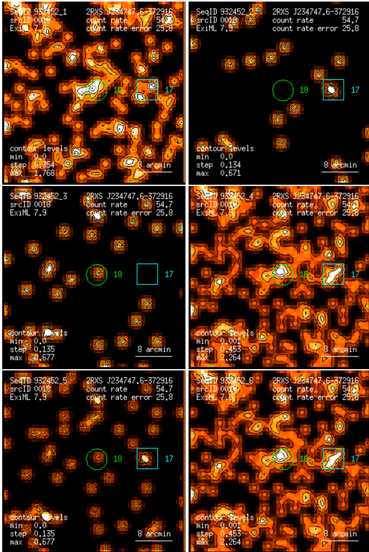
Figure 18: RASS 932452: detection 0018: band rate images, Gaussian filter: (1) PSPC channels 11 – 41, (2) 52 – 90, (3) 91 – 201, (4) 11 – 235, (5) 52 – 201, (6) 11 – 201. Broad band rates in counts/ks. Band rate contour levels in counts/ks/arcmin 2 .
