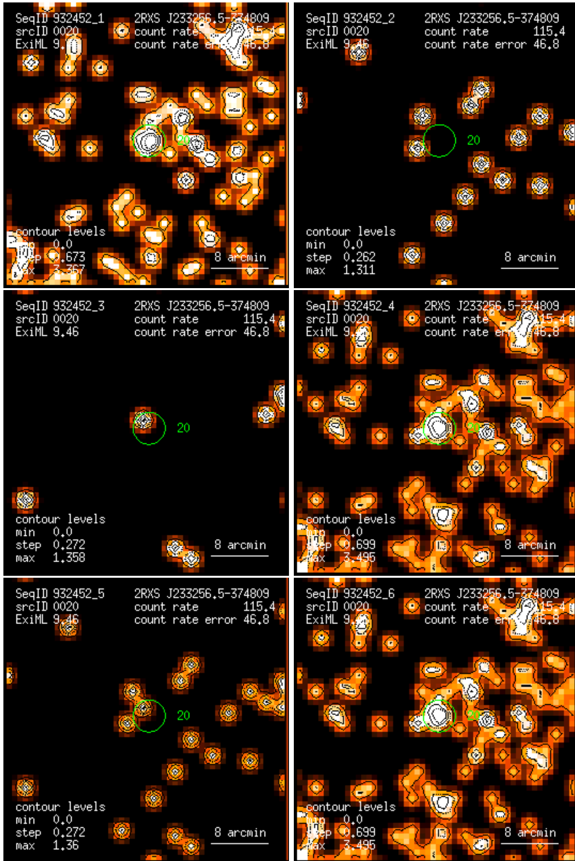
Figure 20: RASS 932452: detection 0020: band rate images, Gaussian filter: (1) PSPC channels 11 – 41, (2) 52 – 90, (3) 91 – 201, (4) 11 – 235, (5) 52 – 201, (6) 11 – 201. Broad band rates in counts/ks. Band rate contour levels in counts/ks/arcmin 2 .
