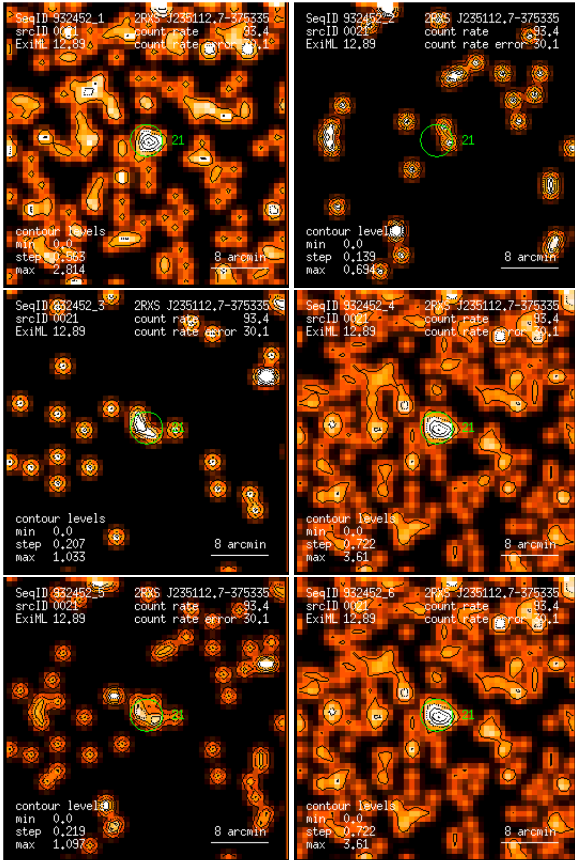
Figure 21: RASS 932452: detection 0021: band rate images, Gaussian filter: (1) PSPC channels 11 – 41, (2) 52 – 90, (3) 91 – 201, (4) 11 – 235, (5) 52 – 201, (6) 11 – 201. Broad band rates in counts/ks. Band rate contour levels in counts/ks/arcmin 2 .
