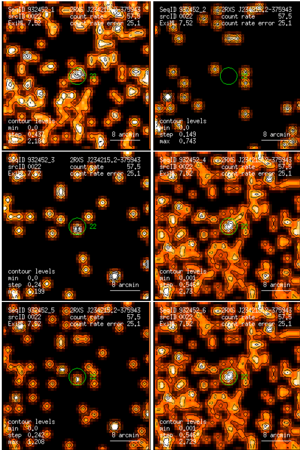
Figure 22: RASS 932452: detection 0022: band rate images, Gaussian filter: (1) PSPC channels 11 – 41, (2) 52 – 90, (3) 91 – 201, (4) 11 – 235, (5) 52 – 201, (6) 11 – 201. Broad band rates in counts/ks. Band rate contour levels in counts/ks/arcmin 2 .
