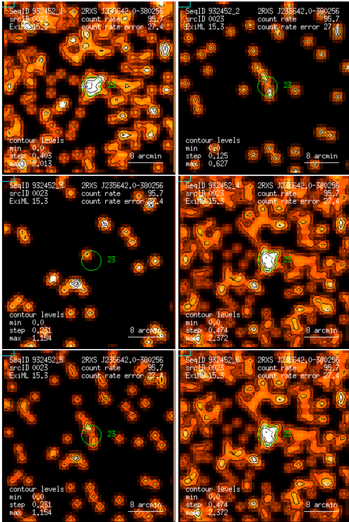
Figure 23: RASS 932452: detection 0023: band rate images, Gaussian filter: (1) PSPC channels 11 – 41, (2) 52 – 90, (3) 91 – 201, (4) 11 – 235, (5) 52 – 201, (6) 11 – 201. Broad band rates in counts/ks. Band rate contour levels in counts/ks/arcmin 2 .
