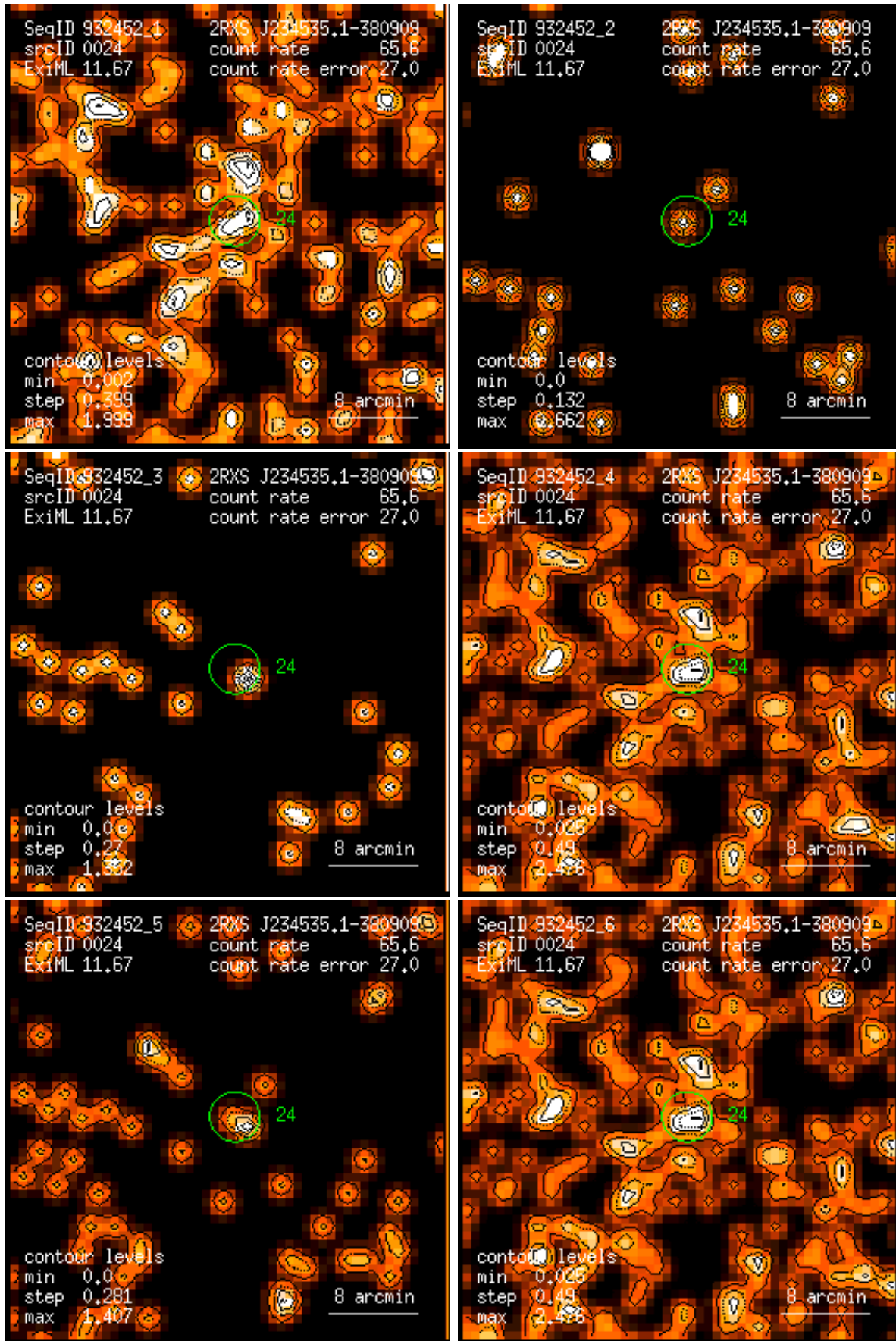
Figure 24: RASS 932452: detection 0024: band rate images, Gaussian filter: (1) PSPC channels 11 – 41, (2) 52 – 90, (3) 91 – 201, (4) 11 – 235, (5) 52 – 201, (6) 11 – 201. Broad band rates in counts/ks. Band rate contour levels in counts/ks/arcmin 2 .
