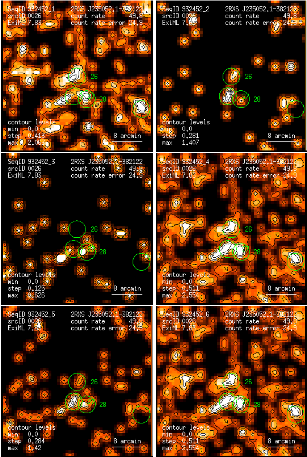
Figure 26: RASS 932452: detection 0026: band rate images, Gaussian filter: (1) PSPC channels 11 – 41, (2) 52 – 90, (3) 91 – 201, (4) 11 – 235, (5) 52 – 201, (6) 11 – 201. Broad band rates in counts/ks. Band rate contour levels in counts/ks/arcmin 2 .
