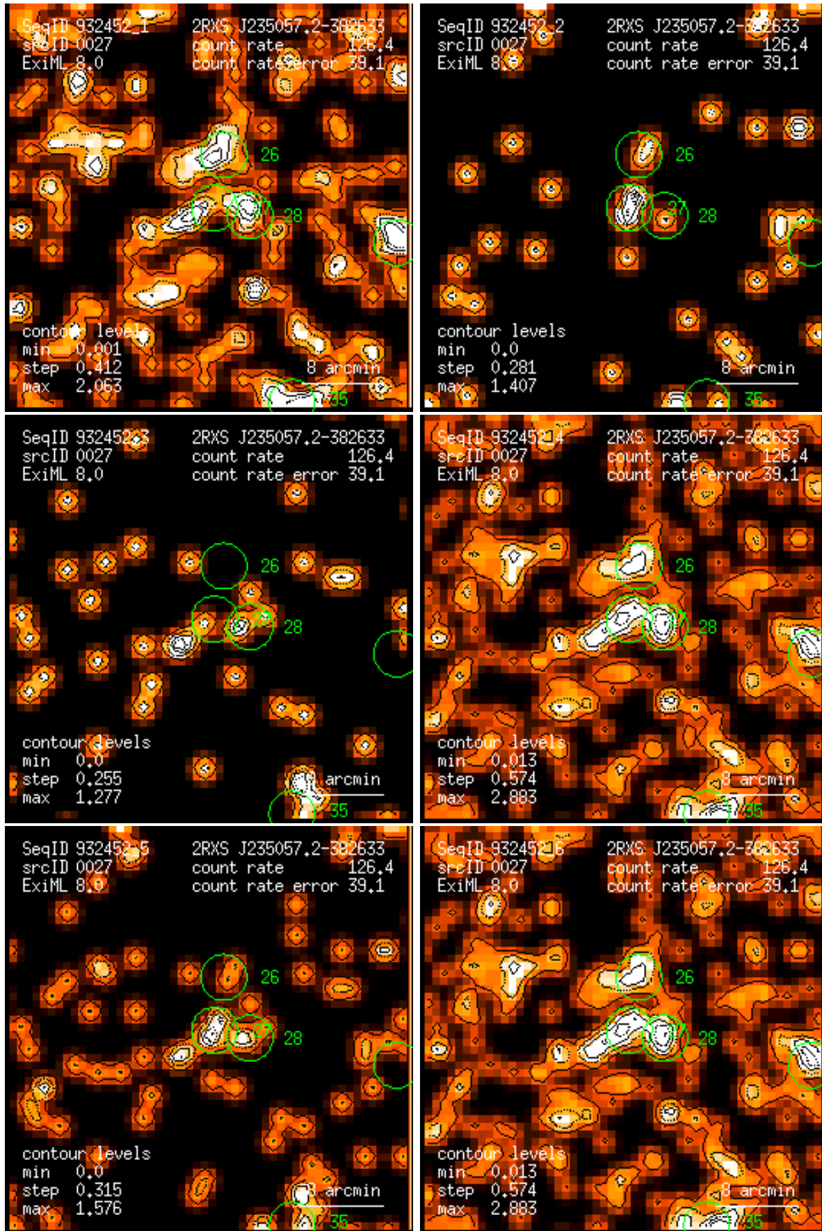
Figure 27: RASS 932452: detection 0027: band rate images, Gaussian filter: (1) PSPC channels 11 – 41, (2) 52 – 90, (3) 91 – 201, (4) 11 – 235, (5) 52 – 201, (6) 11 – 201. Broad band rates in counts/ks. Band rate contour levels in counts/ks/arcmin 2 .
