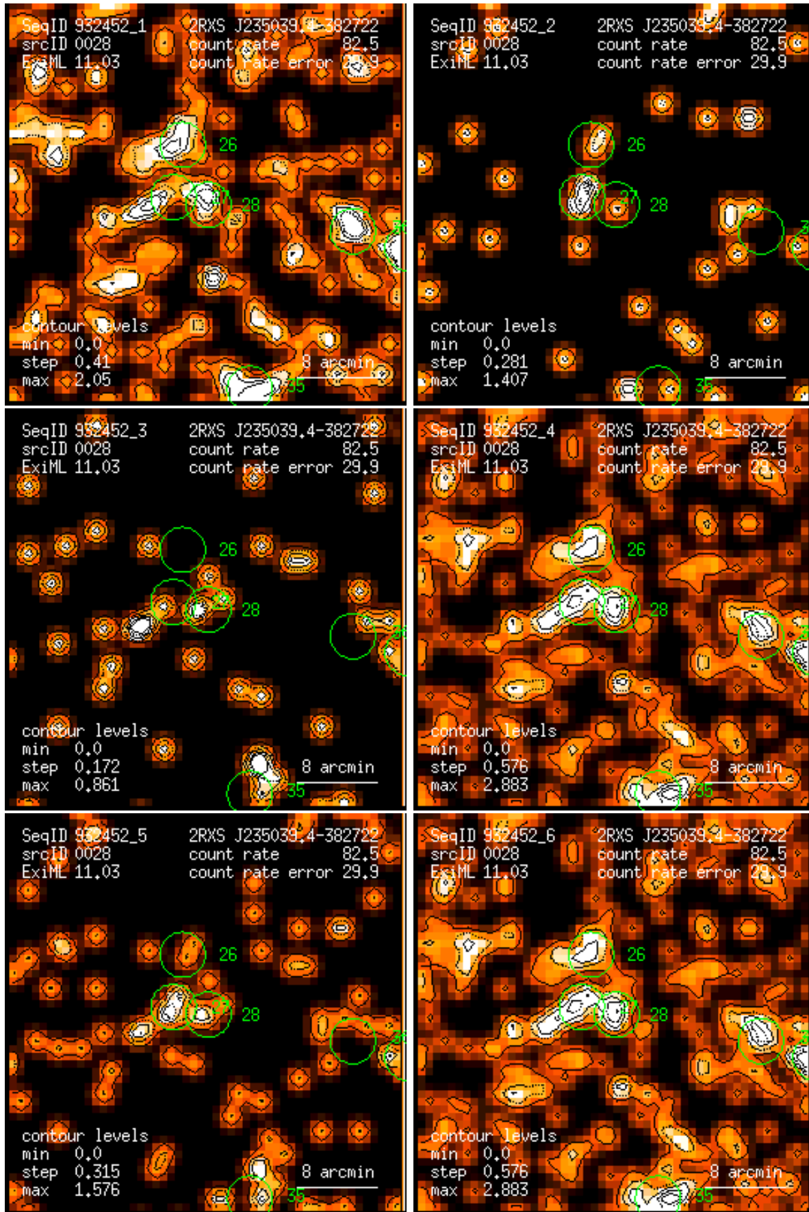
Figure 28: RASS 932452: detection 0028: band rate images, Gaussian filter: (1) PSPC channels 11 – 41, (2) 52 – 90, (3) 91 – 201, (4) 11 – 235, (5) 52 – 201, (6) 11 – 201. Broad band rates in counts/ks. Band rate contour levels in counts/ks/arcmin 2 .
