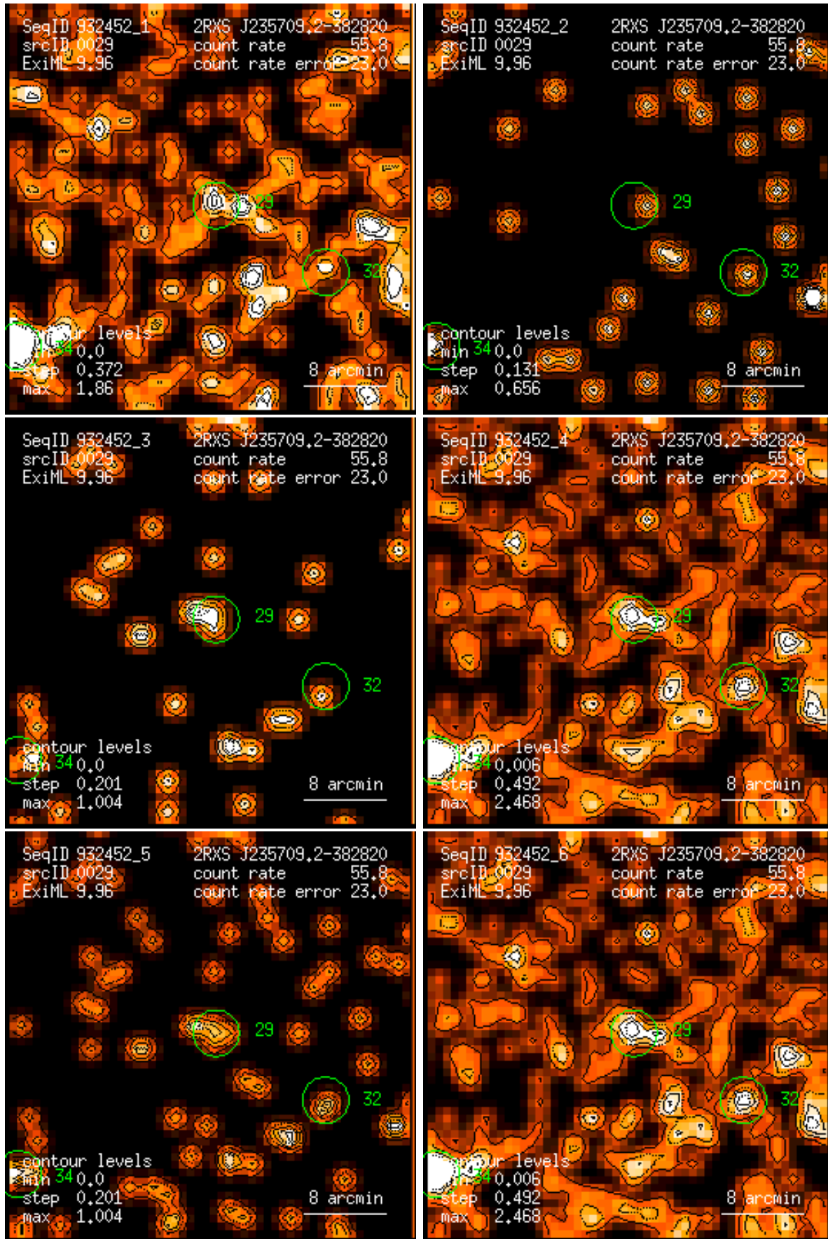
Figure 29: RASS 932452: detection 0029: band rate images, Gaussian filter: (1) PSPC channels 11 – 41, (2) 52 – 90, (3) 91 – 201, (4) 11 – 235, (5) 52 – 201, (6) 11 – 201. Broad band rates in counts/ks. Band rate contour levels in counts/ks/arcmin 2 .
