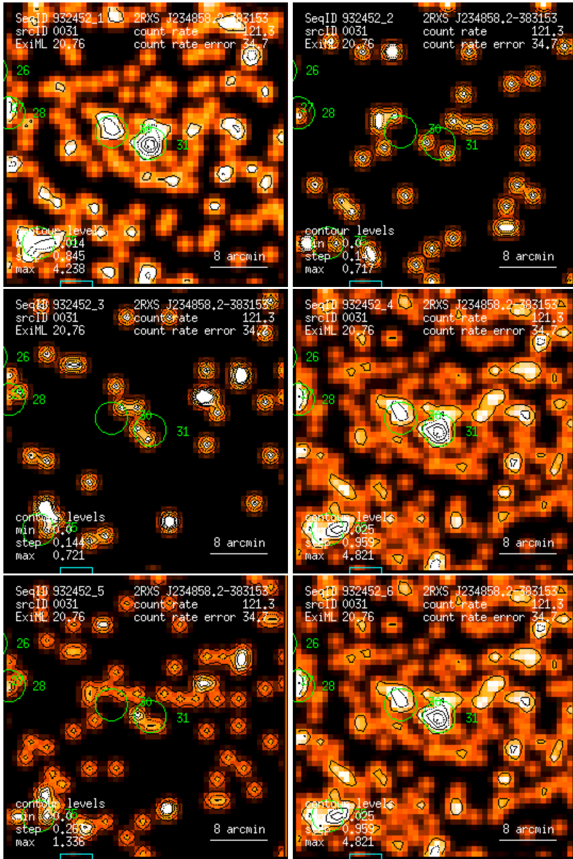
Figure 31: RASS 932452: detection 0031: band rate images, Gaussian filter: (1) PSPC channels 11 – 41, (2) 52 – 90, (3) 91 – 201, (4) 11 – 235, (5) 52 – 201, (6) 11 – 201. Broad band rates in counts/ks. Band rate contour levels in counts/ks/arcmin 2 .
