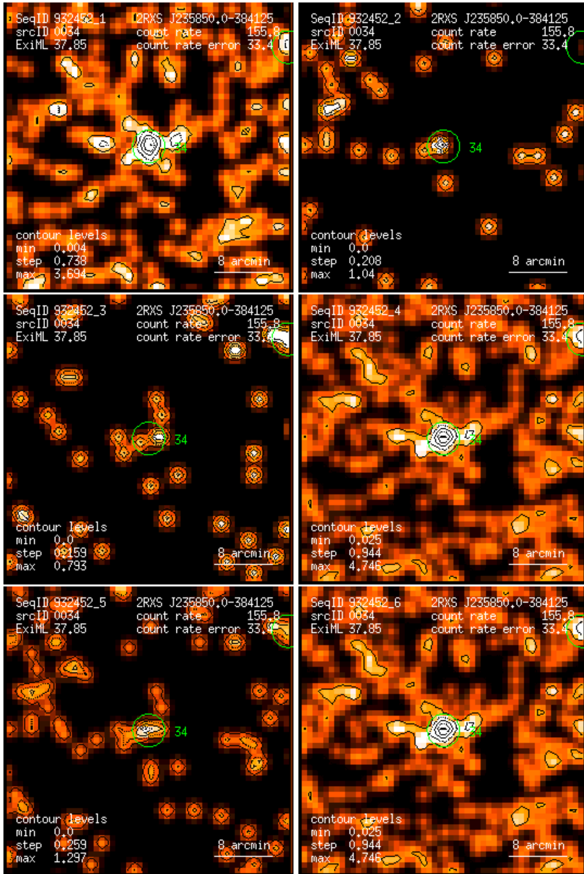
Figure 34: RASS 932452: detection 0034: band rate images, Gaussian filter: (1) PSPC channels 11 – 41, (2) 52 – 90, (3) 91 – 201, (4) 11 – 235, (5) 52 – 201, (6) 11 – 201. Broad band rates in counts/ks. Band rate contour levels in counts/ks/arcmin 2 .
