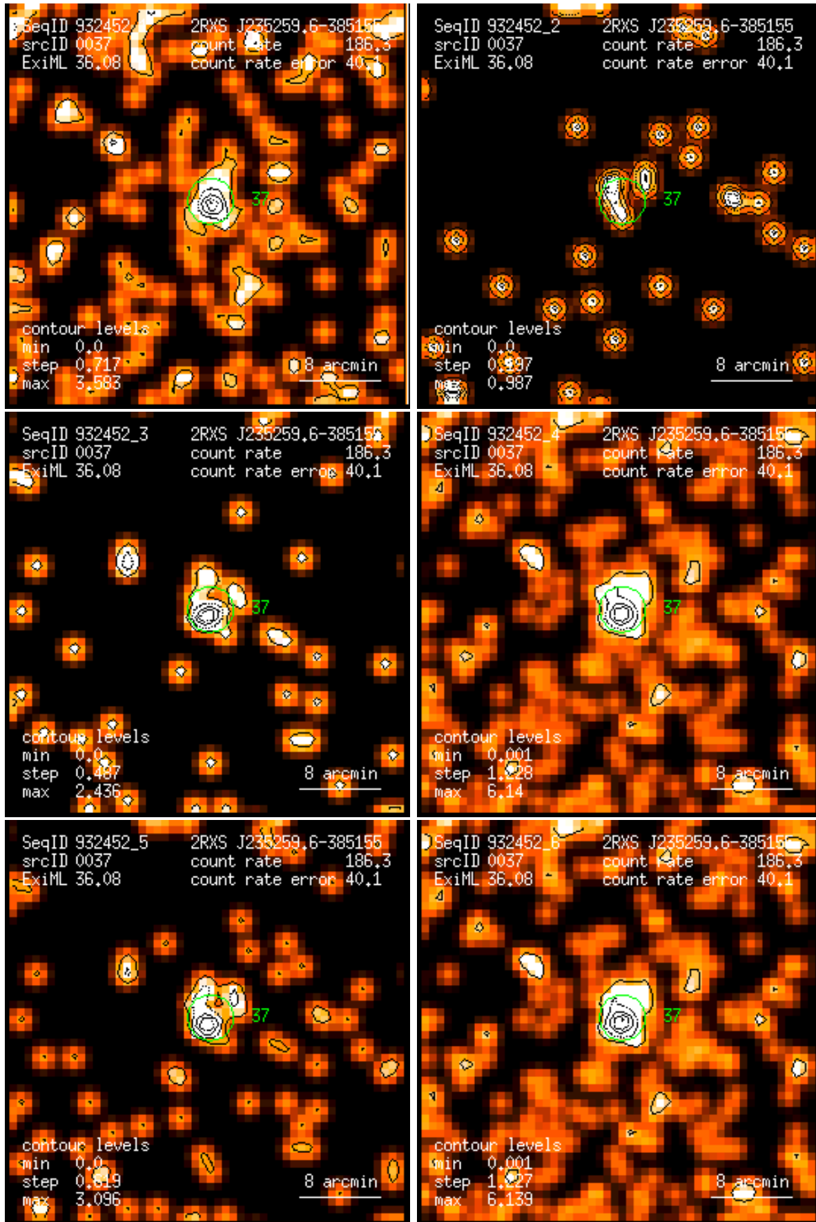
Figure 37: RASS 932452: detection 0037: band rate images, Gaussian filter: (1) PSPC channels 11 – 41, (2) 52 – 90, (3) 91 – 201, (4) 11 – 235, (5) 52 – 201, (6) 11 – 201. Broad band rates in counts/ks. Band rate contour levels in counts/ks/arcmin 2 .
