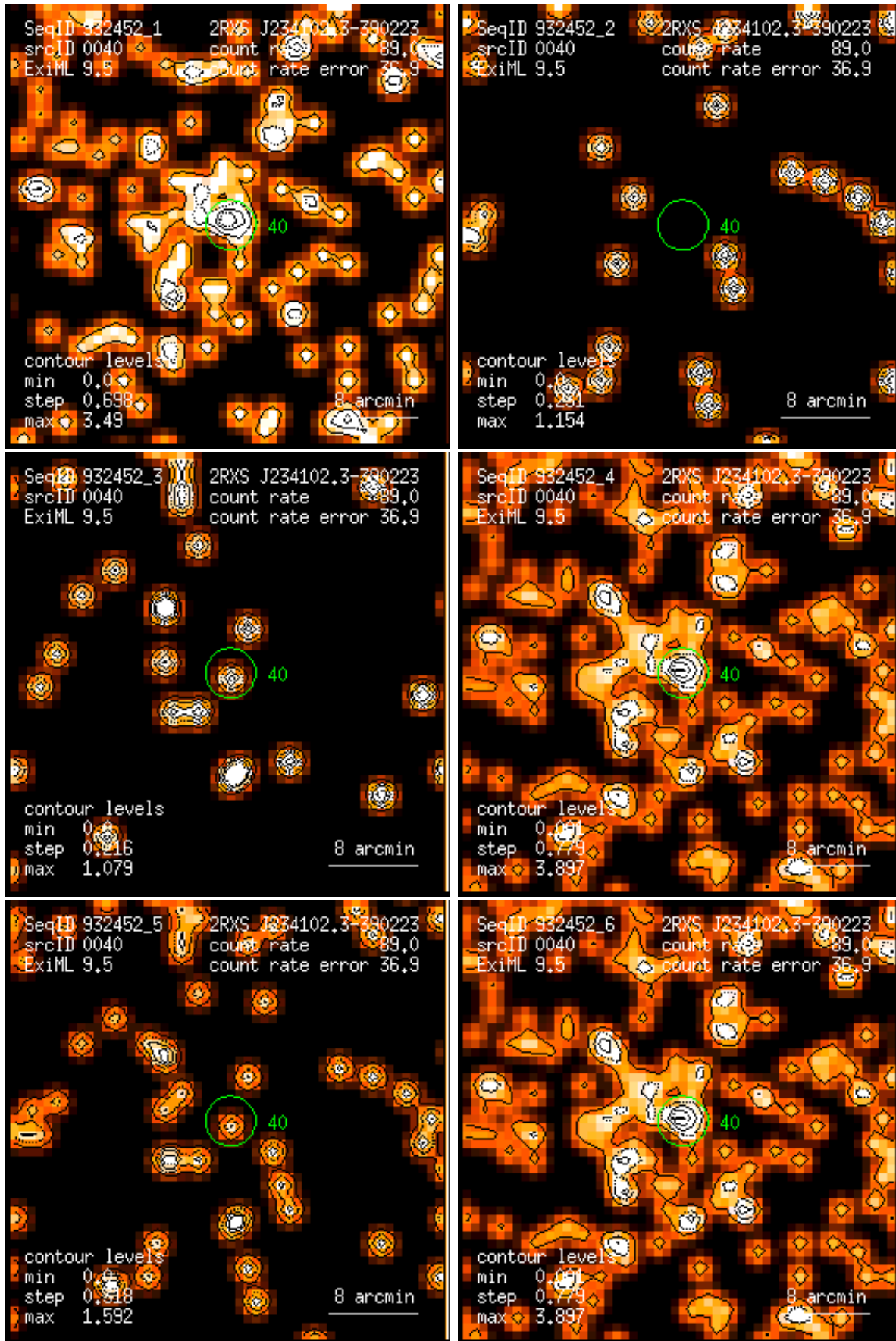
Figure 40: RASS 932452: detection 0040: band rate images, Gaussian filter: (1) PSPC channels 11 – 41, (2) 52 – 90, (3) 91 – 201, (4) 11 – 235, (5) 52 – 201, (6) 11 – 201. Broad band rates in counts/ks. Band rate contour levels in counts/ks/arcmin 2 .
