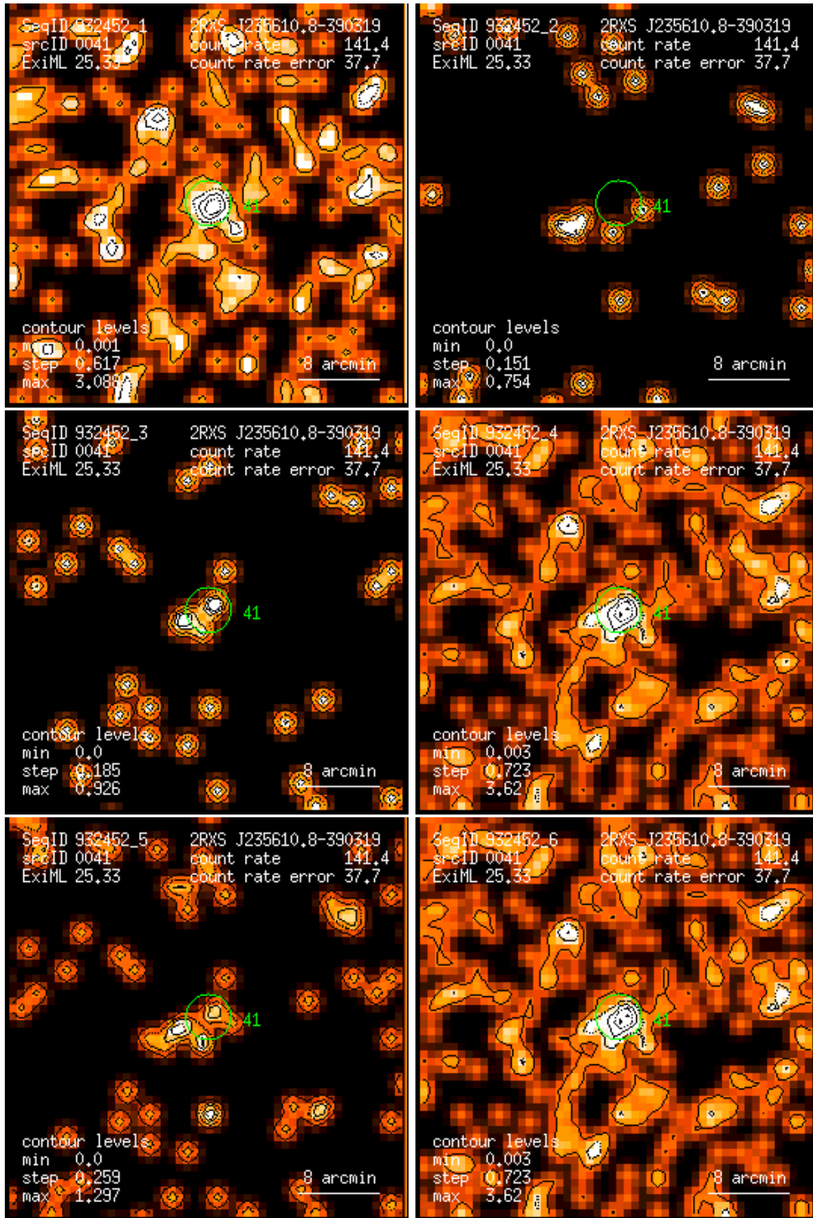
Figure 41: RASS 932452: detection 0041: band rate images, Gaussian filter: (1) PSPC channels 11 – 41, (2) 52 – 90, (3) 91 – 201, (4) 11 – 235, (5) 52 – 201, (6) 11 – 201. Broad band rates in counts/ks. Band rate contour levels in counts/ks/arcmin 2 .
