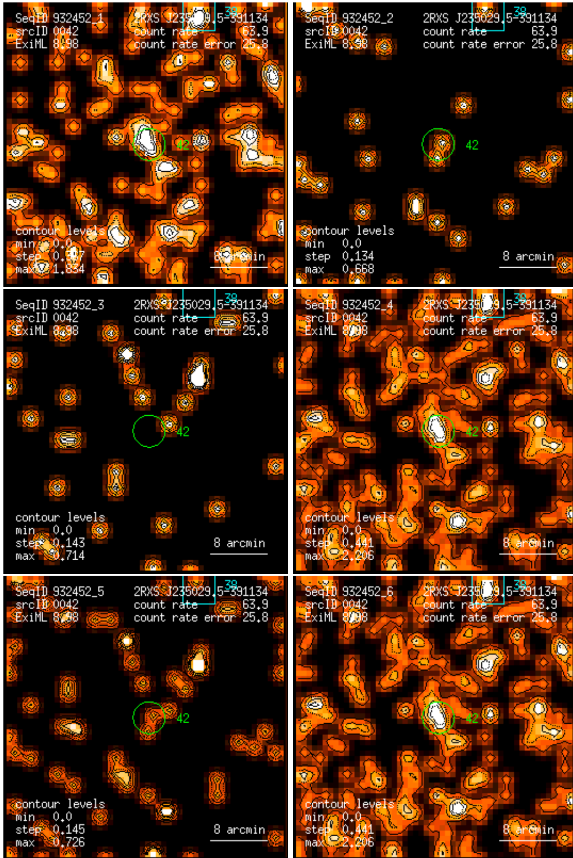
Figure 42: RASS 932452: detection 0042: band rate images, Gaussian filter: (1) PSPC channels 11 – 41, (2) 52 – 90, (3) 91 – 201, (4) 11 – 235, (5) 52 – 201, (6) 11 – 201. Broad band rates in counts/ks. Band rate contour levels in counts/ks/arcmin 2 .
