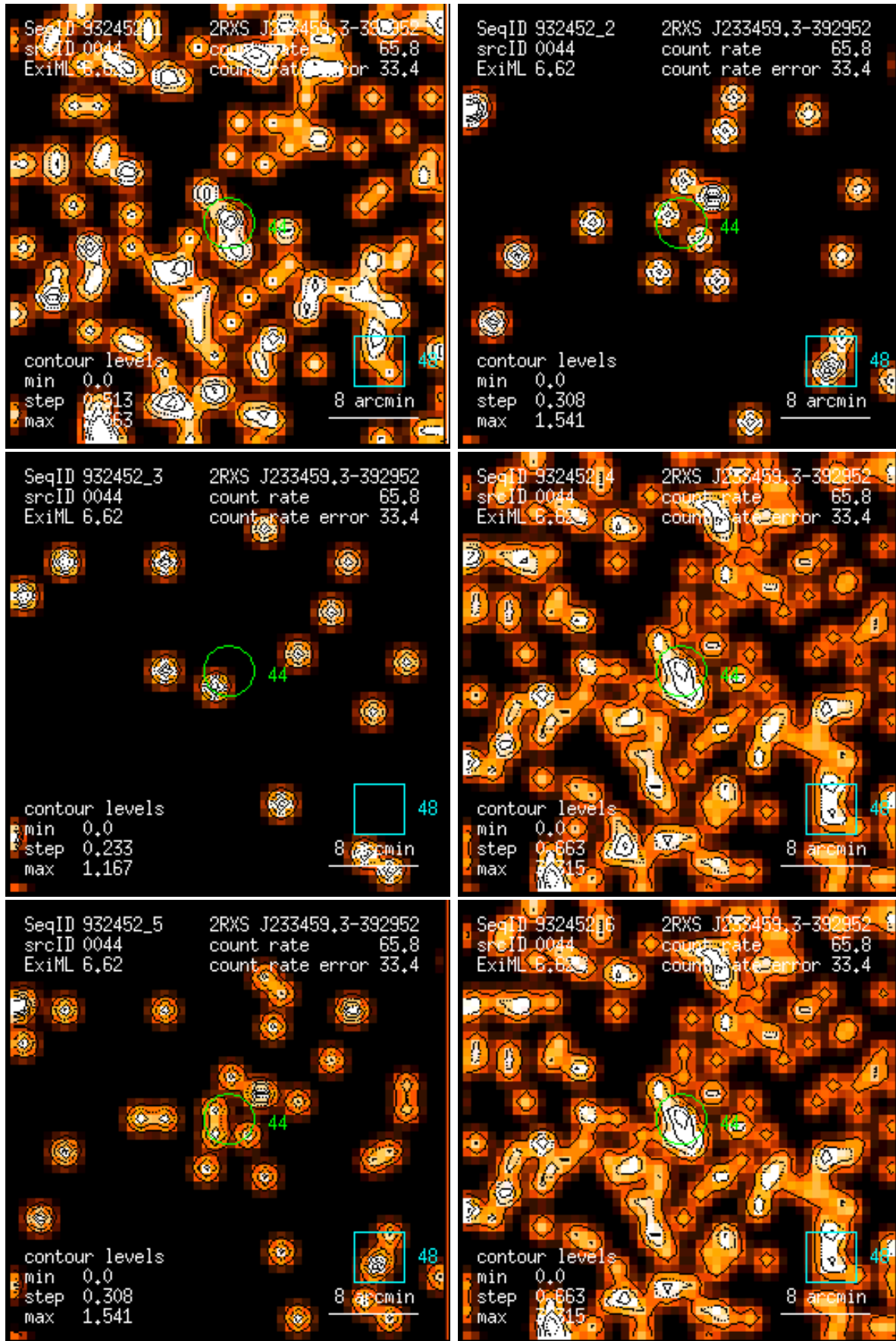
Figure 44: RASS 932452: detection 0044: band rate images, Gaussian filter: (1) PSPC channels 11 – 41, (2) 52 – 90, (3) 91 – 201, (4) 11 – 235, (5) 52 – 201, (6) 11 – 201. Broad band rates in counts/ks. Band rate contour levels in counts/ks/arcmin 2 .
