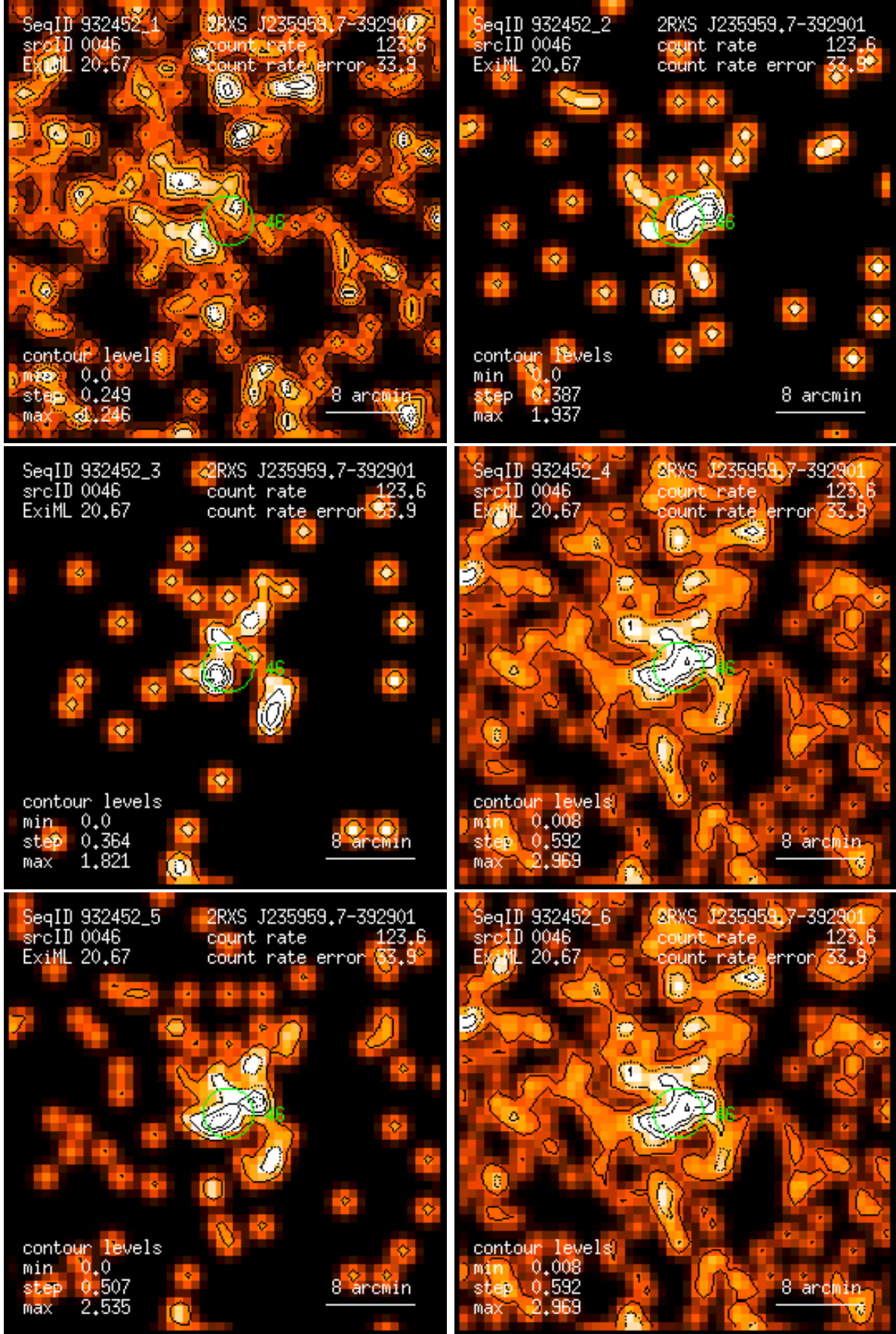
Figure 46: RASS 932452: detection 0046: band rate images, Gaussian filter: (1) PSPC channels 11 – 41, (2) 52 – 90, (3) 91 – 201, (4) 11 – 235, (5) 52 – 201, (6) 11 – 201. Broad band rates in counts/ks. Band rate contour levels in counts/ks/arcmin 2 .
