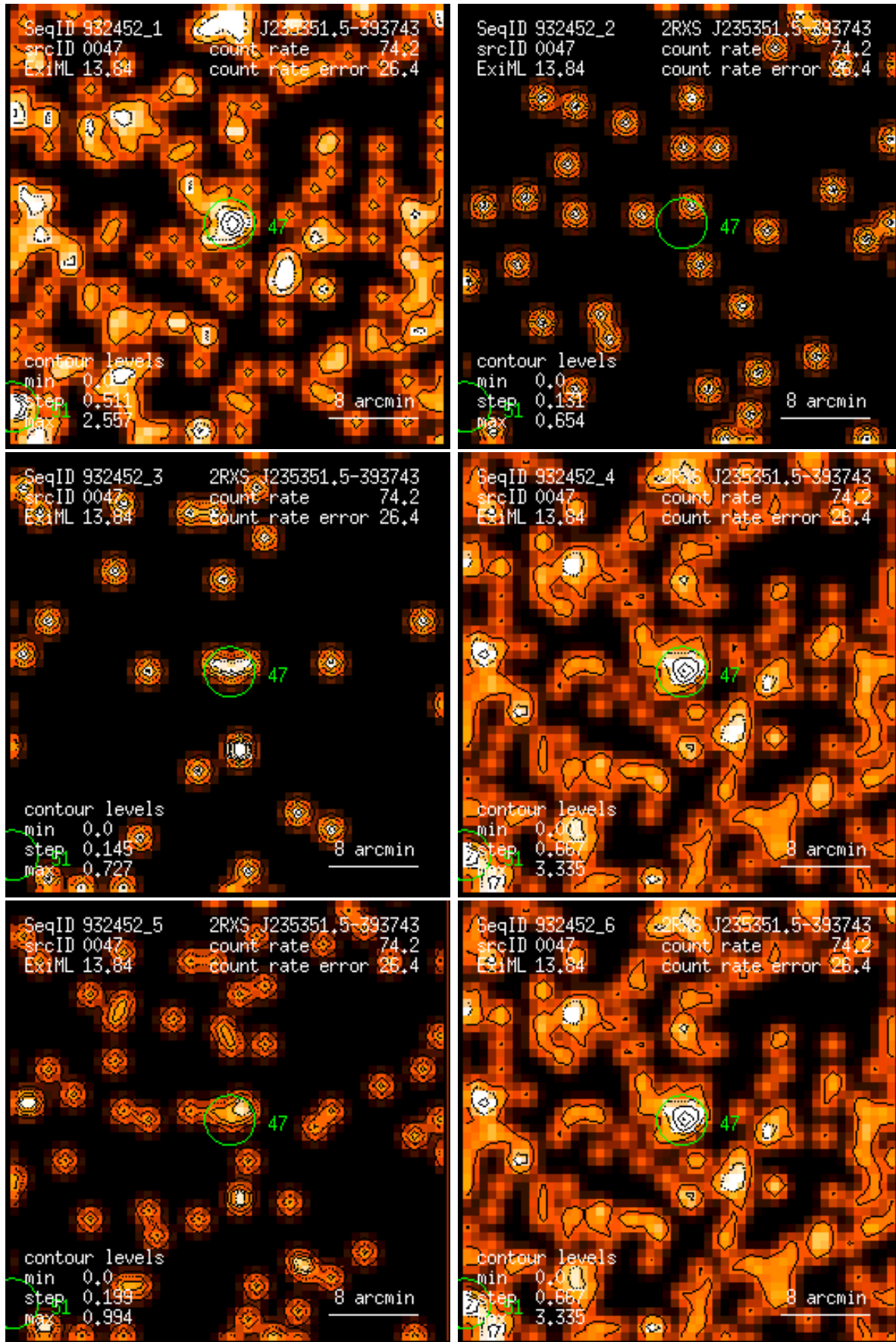
Figure 47: RASS 932452: detection 0047: band rate images, Gaussian filter: (1) PSPC channels 11 – 41, (2) 52 – 90, (3) 91 – 201, (4) 11 – 235, (5) 52 – 201, (6) 11 – 201. Broad band rates in counts/ks. Band rate contour levels in counts/ks/arcmin 2 .
