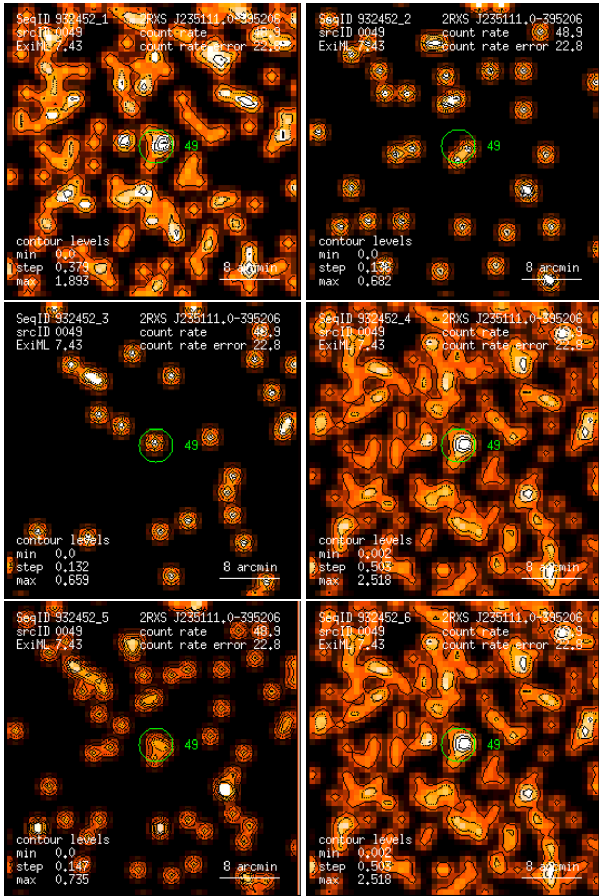
Figure 49: RASS 932452: detection 0049: band rate images, Gaussian filter: (1) PSPC channels 11 – 41, (2) 52 – 90, (3) 91 – 201, (4) 11 – 235, (5) 52 – 201, (6) 11 – 201. Broad band rates in counts/ks. Band rate contour levels in counts/ks/arcmin 2 .
