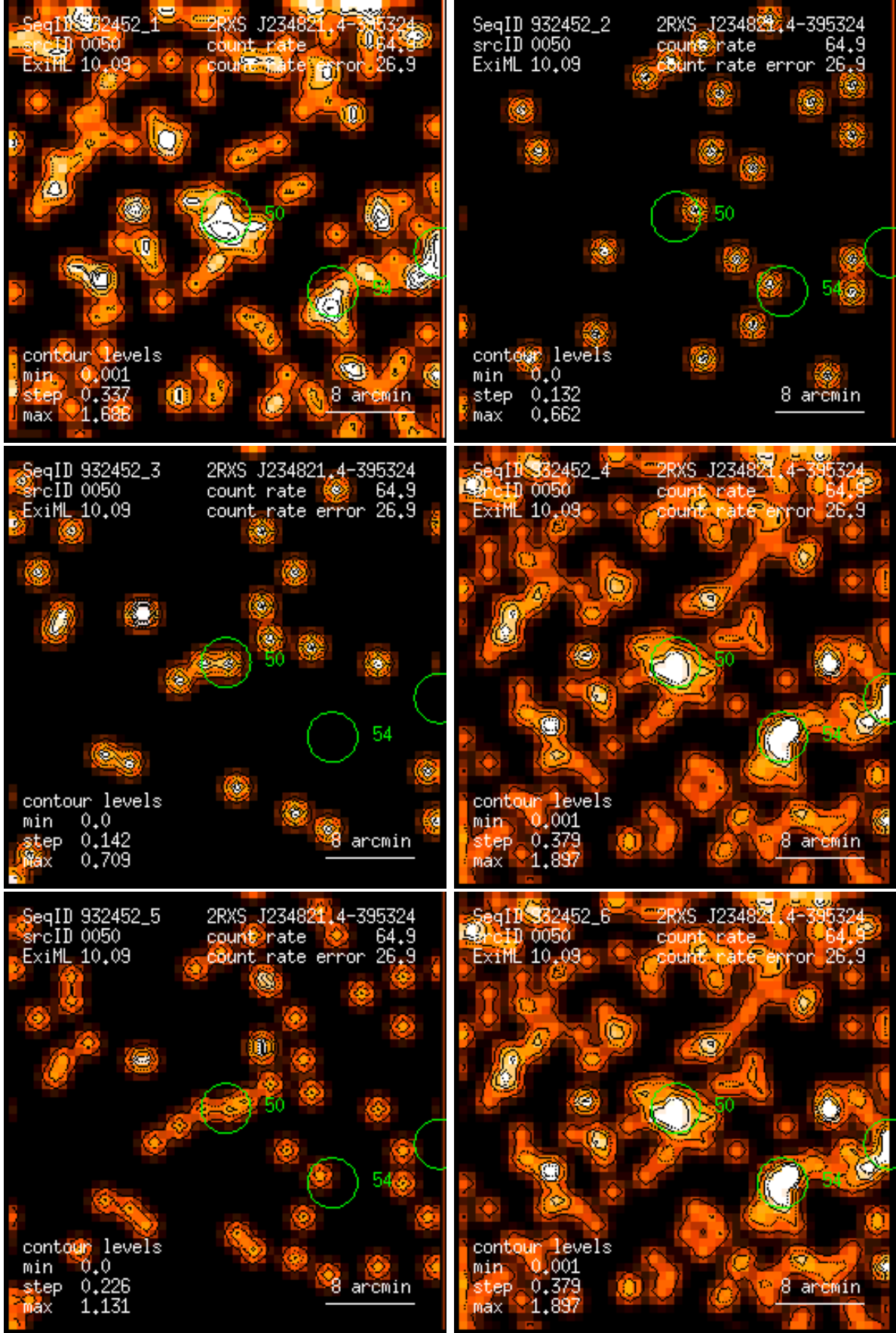
Figure 50: RASS 932452: detection 0050: band rate images, Gaussian filter: (1) PSPC channels 11 – 41, (2) 52 – 90, (3) 91 – 201, (4) 11 – 235, (5) 52 – 201, (6) 11 – 201. Broad band rates in counts/ks. Band rate contour levels in counts/ks/arcmin 2 .
