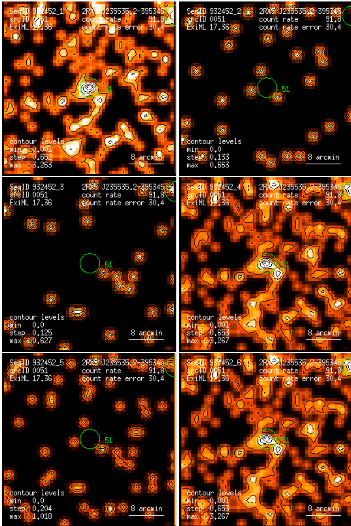
Figure 51: RASS 932452: detection 0051: band rate images, Gaussian filter: (1) PSPC channels 11 – 41, (2) 52 – 90, (3) 91 – 201, (4) 11 – 235, (5) 52 – 201, (6) 11 – 201. Broad band rates in counts/ks. Band rate contour levels in counts/ks/arcmin 2 .
