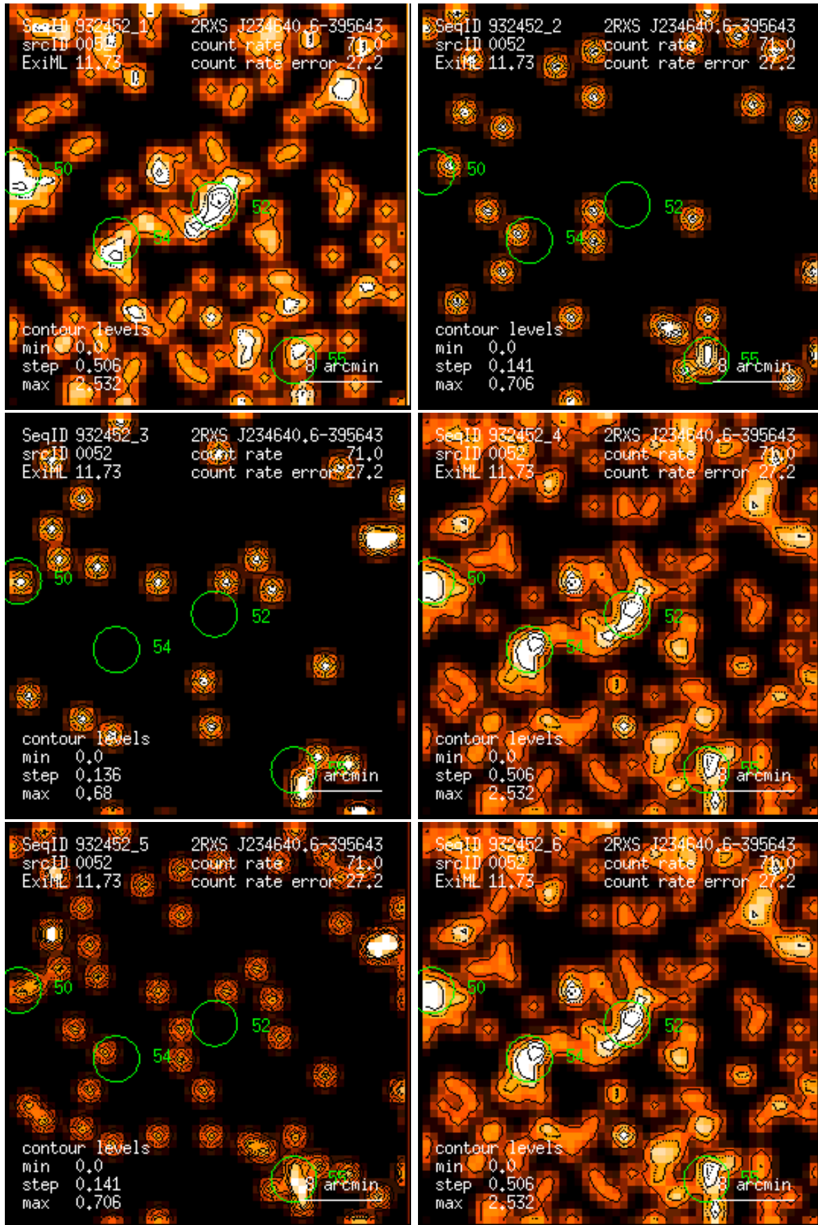
Figure 52: RASS 932452: detection 0052: band rate images, Gaussian filter: (1) PSPC channels 11 – 41, (2) 52 – 90, (3) 91 – 201, (4) 11 – 235, (5) 52 – 201, (6) 11 – 201. Broad band rates in counts/ks. Band rate contour levels in counts/ks/arcmin 2 .
