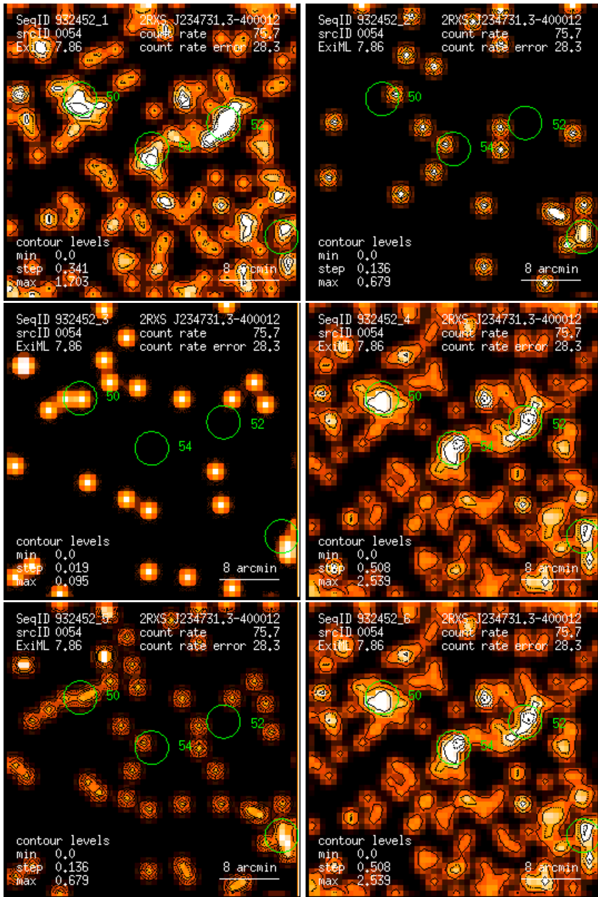
Figure 54: RASS 932452: detection 0054: band rate images, Gaussian filter: (1) PSPC channels 11 – 41, (2) 52 – 90, (3) 91 – 201, (4) 11 – 235, (5) 52 – 201, (6) 11 – 201. Broad band rates in counts/ks. Band rate contour levels in counts/ks/arcmin 2 .
