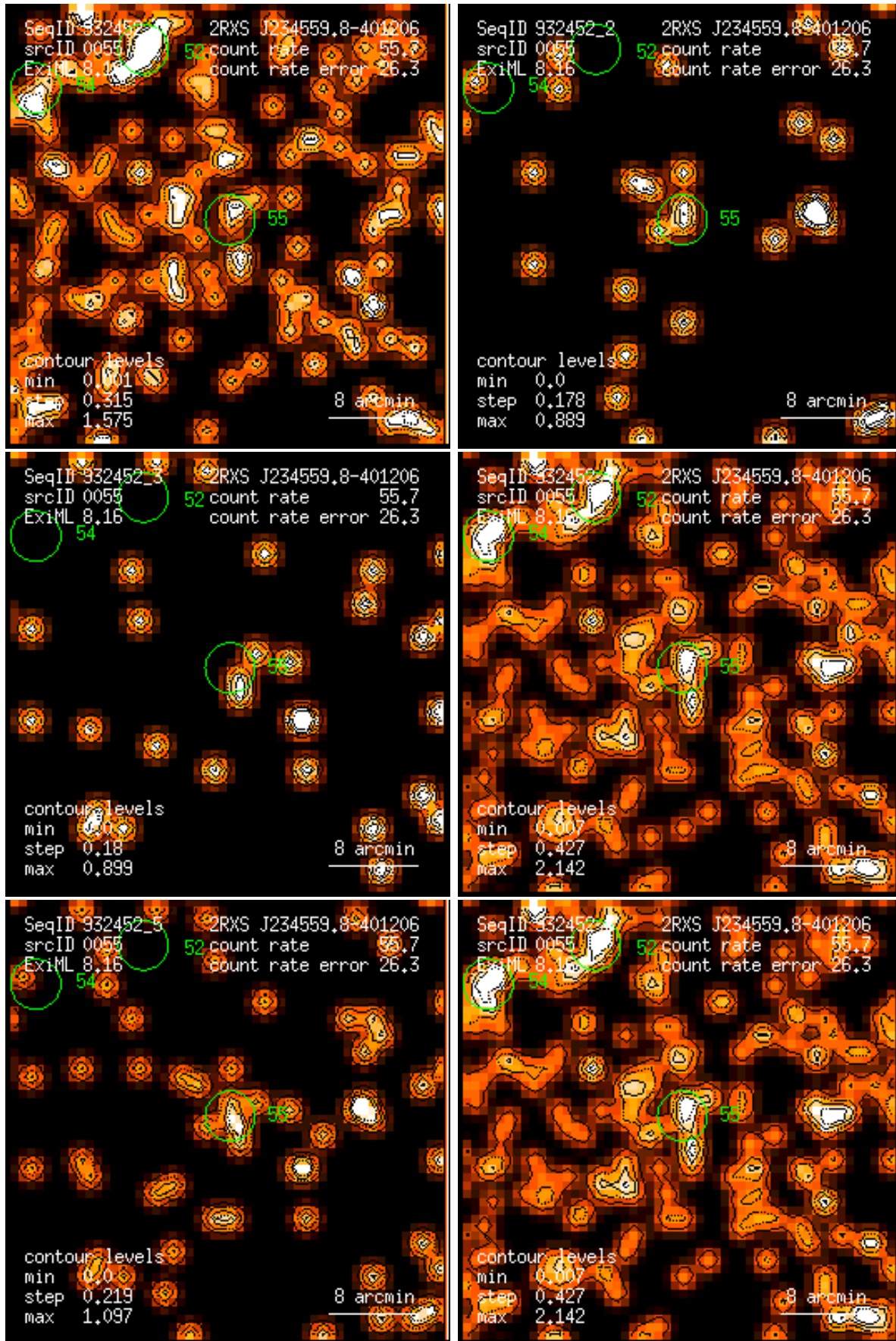
Figure 55: RASS 932452: detection 0055: band rate images, Gaussian filter: (1) PSPC channels 11 – 41, (2) 52 – 90, (3) 91 – 201, (4) 11 – 235, (5) 52 – 201, (6) 11 – 201. Broad band rates in counts/ks. Band rate contour levels in counts/ks/arcmin 2 .
