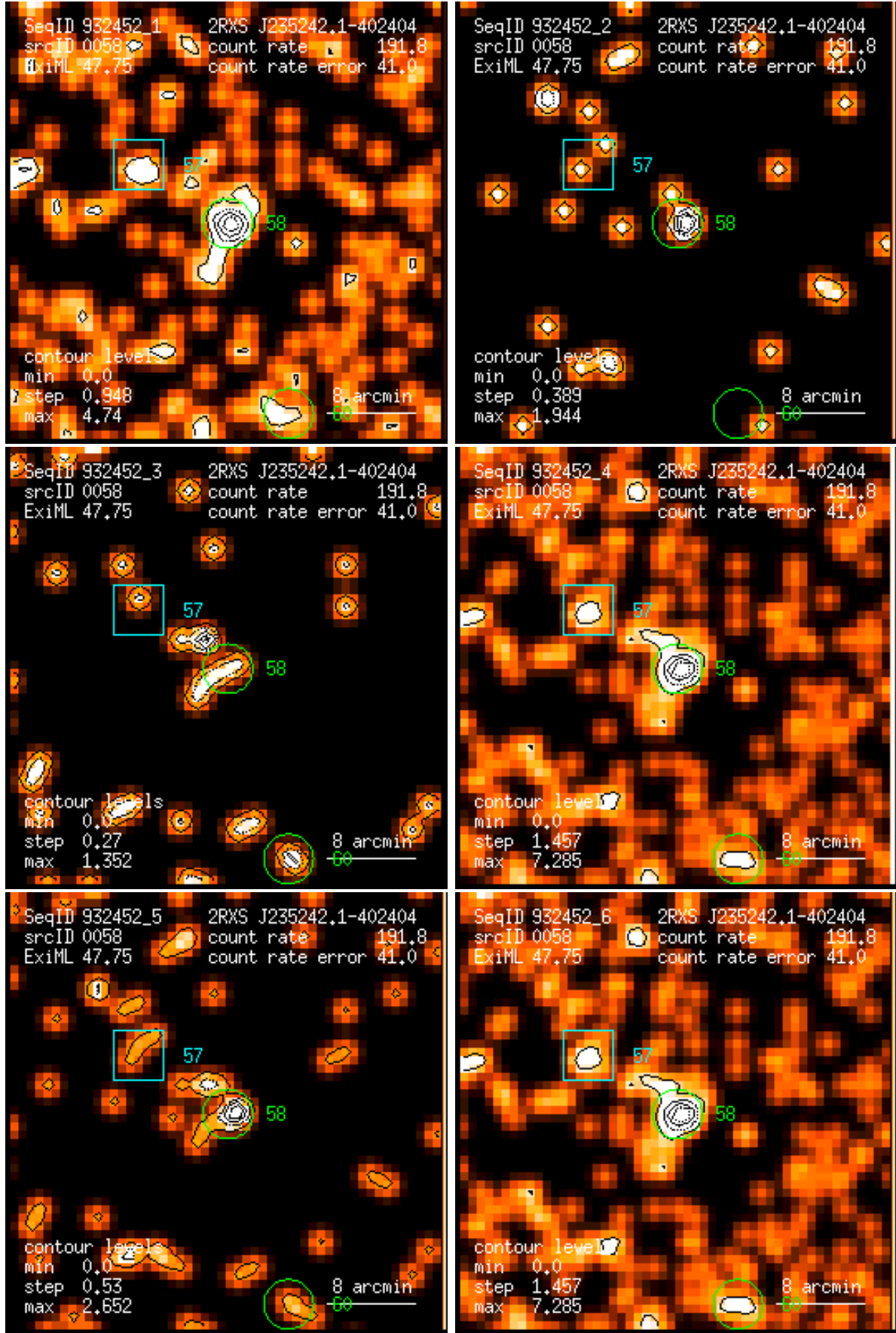
Figure 58: RASS 932452: detection 0058: band rate images, Gaussian filter: (1) PSPC channels 11 – 41, (2) 52 – 90, (3) 91 – 201, (4) 11 – 235, (5) 52 – 201, (6) 11 – 201. Broad band rates in counts/ks. Band rate contour levels in counts/ks/arcmin 2 .
