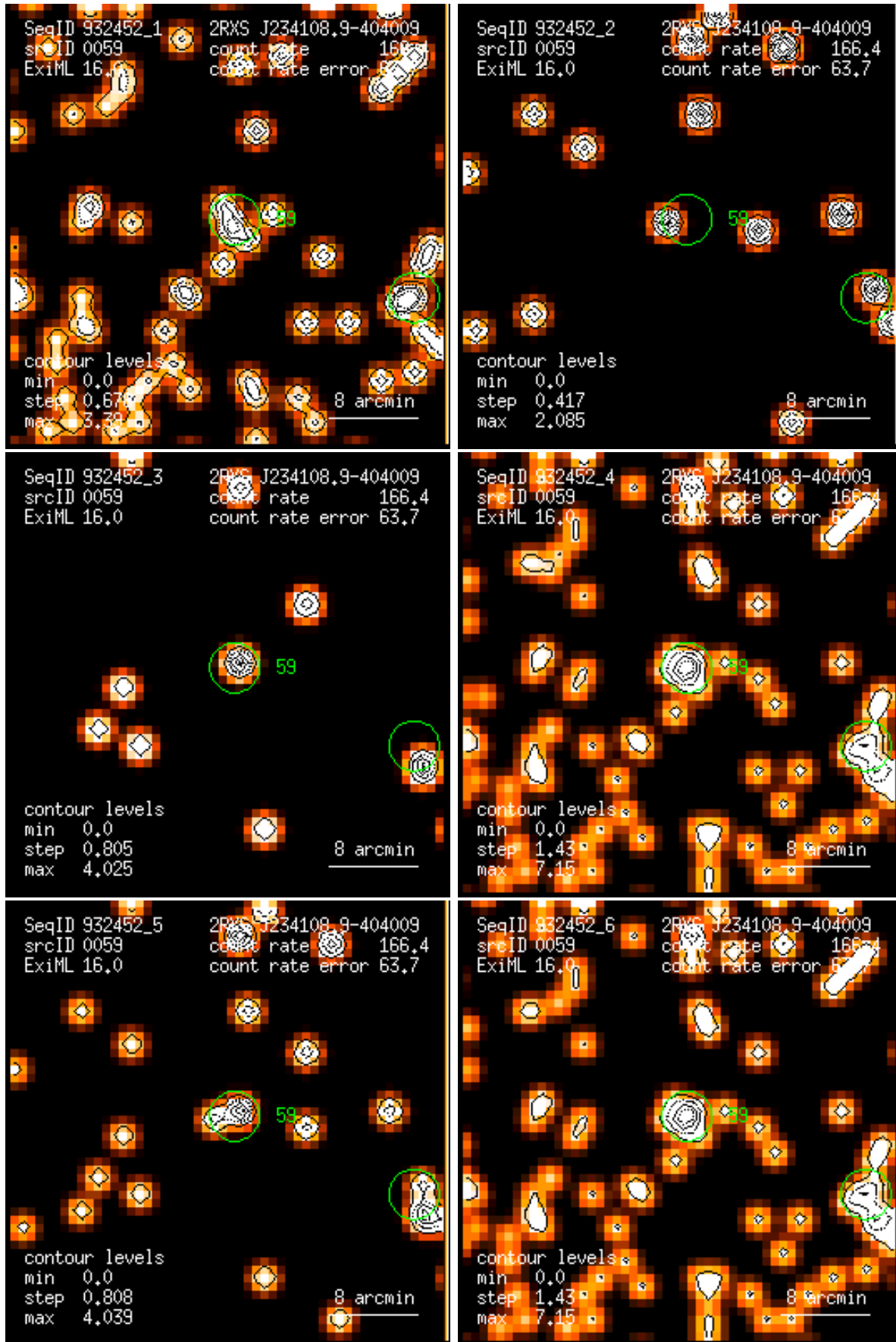
Figure 59: RASS 932452: detection 0059: band rate images, Gaussian filter: (1) PSPC channels 11 – 41, (2) 52 – 90, (3) 91 – 201, (4) 11 – 235, (5) 52 – 201, (6) 11 – 201. Broad band rates in counts/ks. Band rate contour levels in counts/ks/arcmin 2 .
