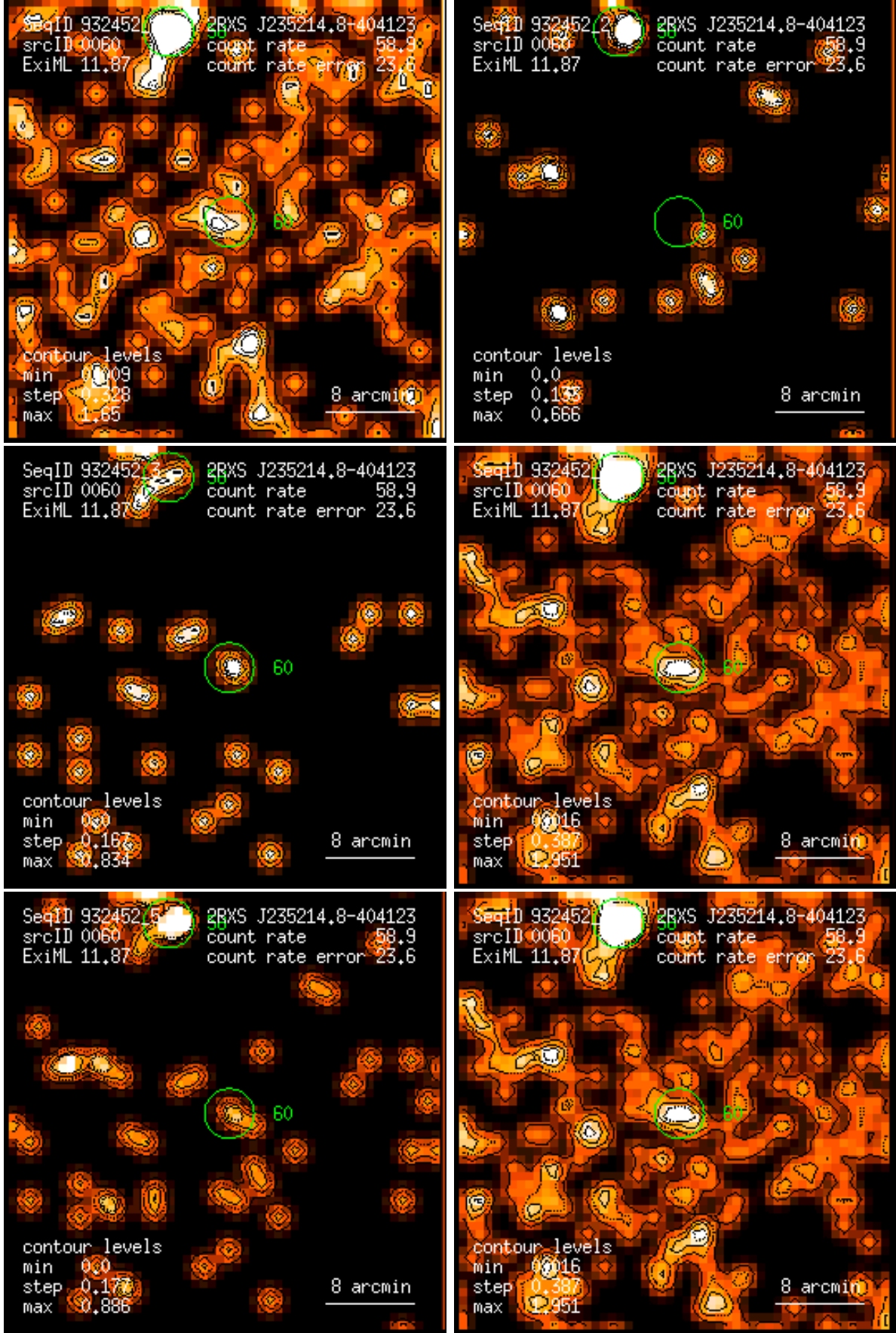
Figure 60: RASS 932452: detection 0060: band rate images, Gaussian filter: (1) PSPC channels 11 – 41, (2) 52 – 90, (3) 91 – 201, (4) 11 – 235, (5) 52 – 201, (6) 11 – 201. Broad band rates in counts/ks. Band rate contour levels in counts/ks/arcmin 2 .
