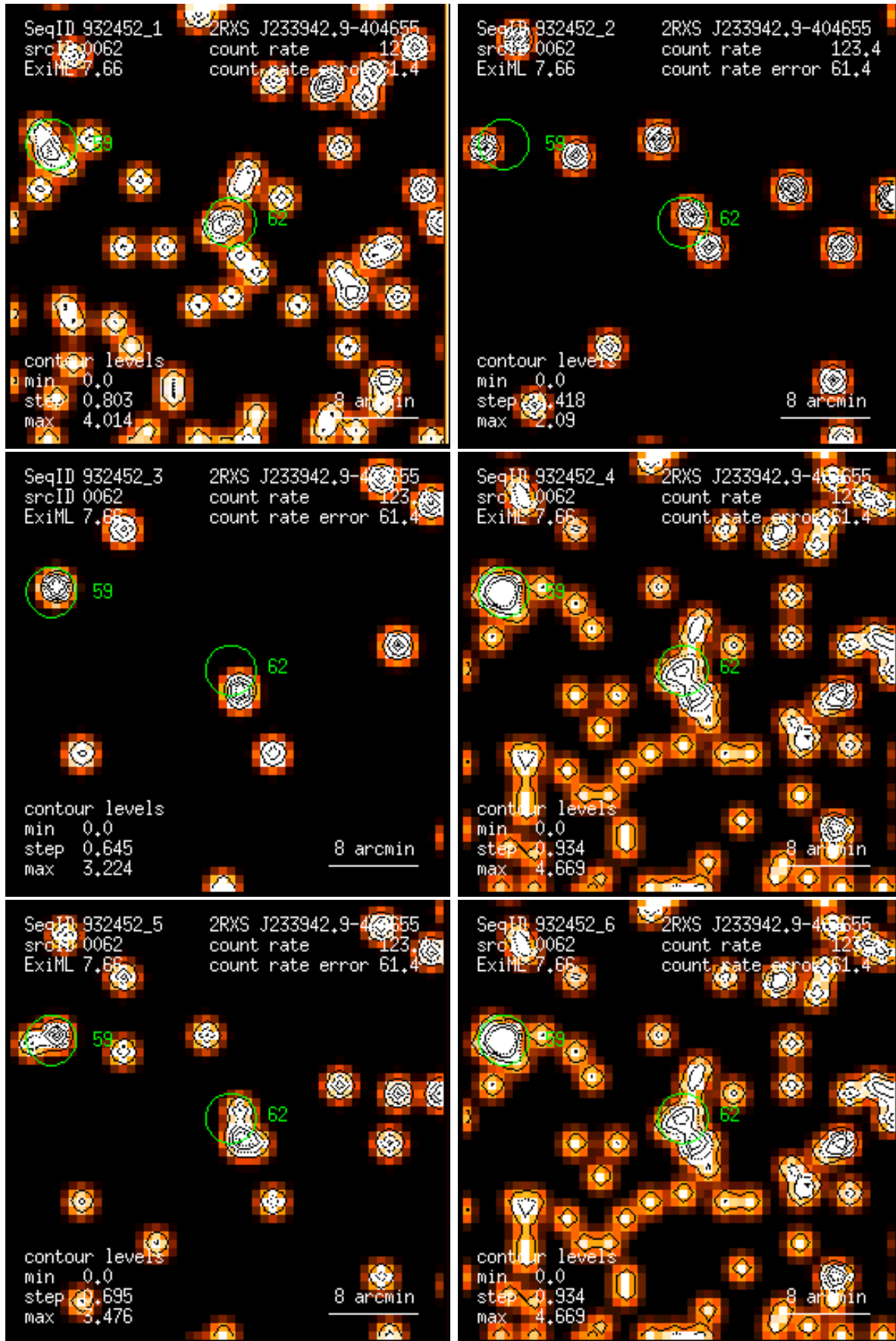
Figure 62: RASS 932452: detection 0062: band rate images, Gaussian filter: (1) PSPC channels 11 – 41, (2) 52 – 90, (3) 91 – 201, (4) 11 – 235, (5) 52 – 201, (6) 11 – 201. Broad band rates in counts/ks. Band rate contour levels in counts/ks/arcmin 2 .
