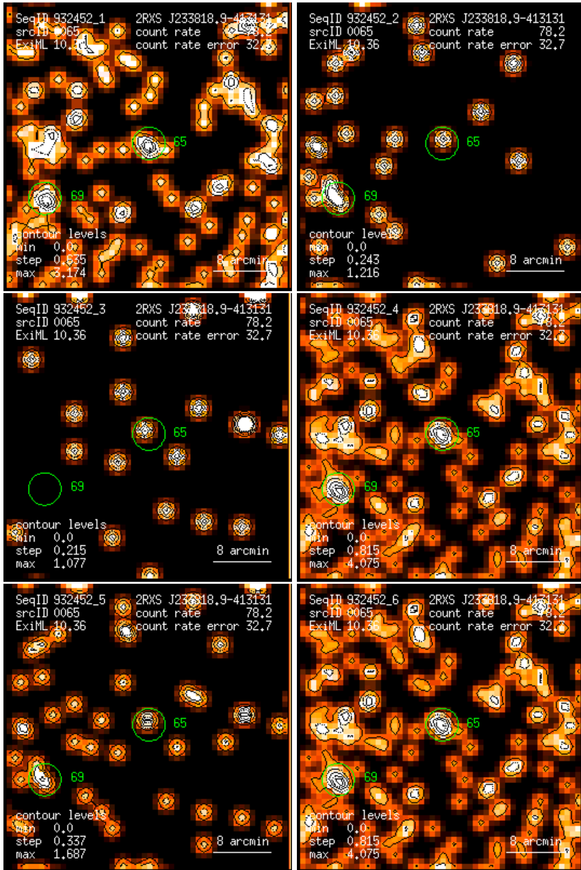
Figure 65: RASS 932452: detection 0065: band rate images, Gaussian filter: (1) PSPC channels 11 – 41, (2) 52 – 90, (3) 91 – 201, (4) 11 – 235, (5) 52 – 201, (6) 11 – 201. Broad band rates in counts/ks. Band rate contour levels in counts/ks/arcmin 2 .
