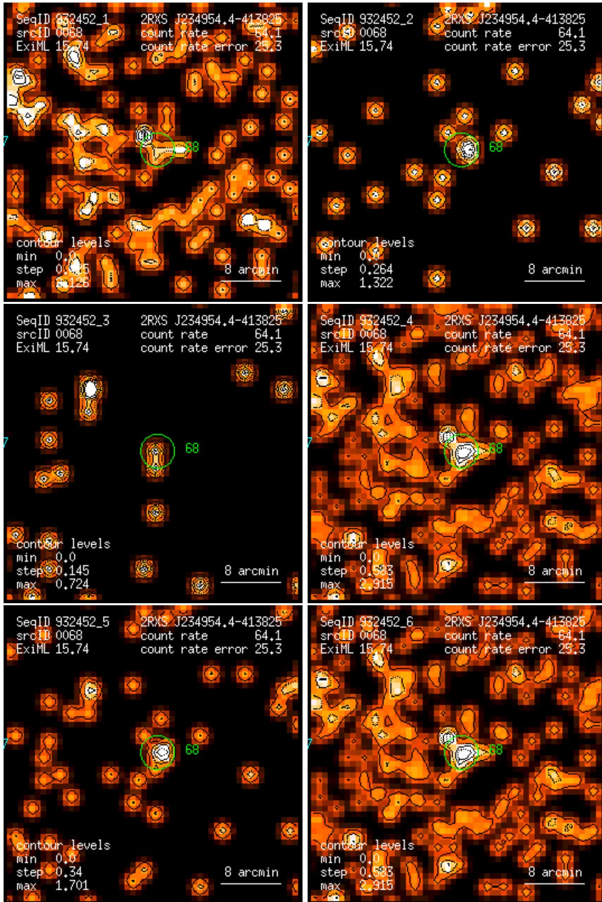
Figure 68: RASS 932452: detection 0068: band rate images, Gaussian filter: (1) PSPC channels 11 – 41, (2) 52 – 90, (3) 91 – 201, (4) 11 – 235, (5) 52 – 201, (6) 11 – 201. Broad band rates in counts/ks. Band rate contour levels in counts/ks/arcmin 2 .
