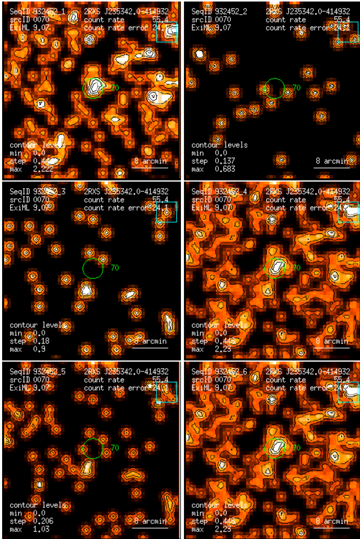
Figure 70: RASS 932452: detection 0070: band rate images, Gaussian filter: (1) PSPC channels 11 – 41, (2) 52 – 90, (3) 91 – 201, (4) 11 – 235, (5) 52 – 201, (6) 11 – 201. Broad band rates in counts/ks. Band rate contour levels in counts/ks/arcmin 2 .
