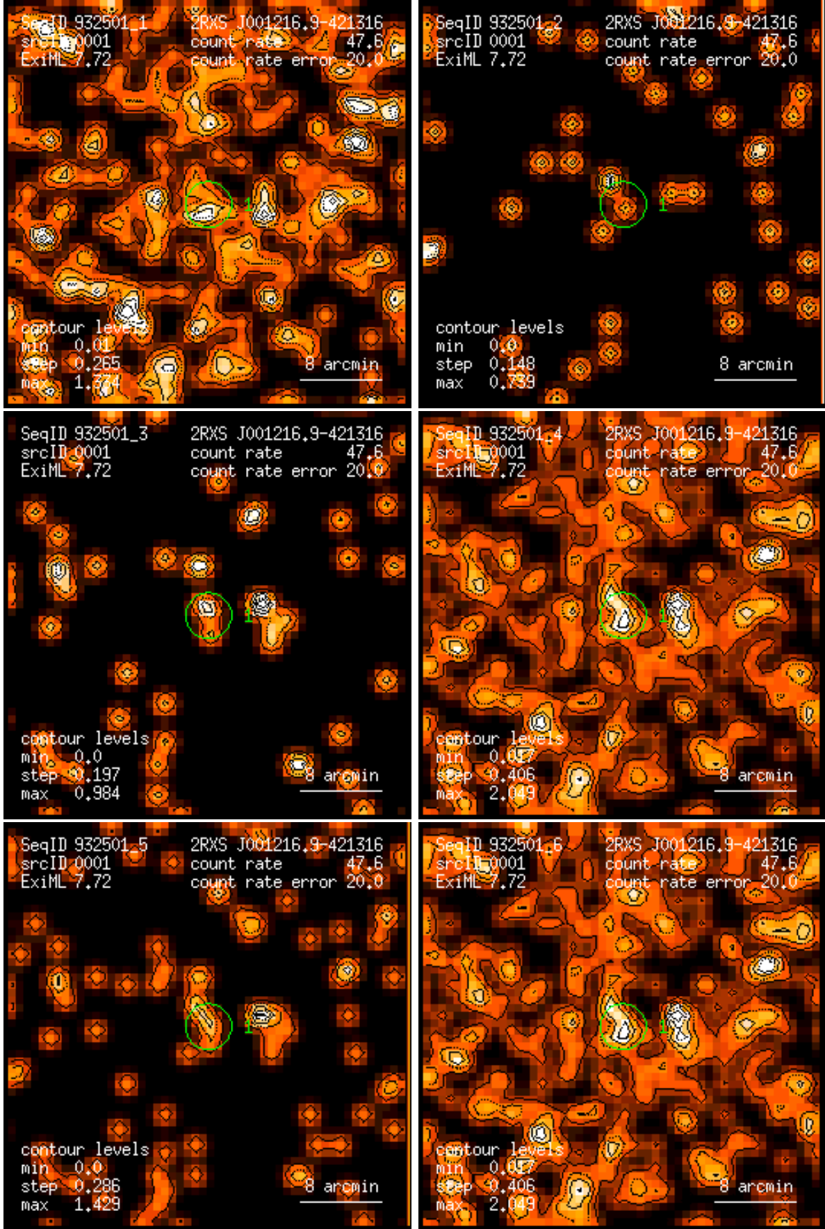
Figure 1: RASS 932501: detection 0001: band rate images, Gaussian filter: (1) PSPC channels 11 – 41, (2) 52 – 90, (3) 91 – 201, (4) 11 – 235, (5) 52 – 201, (6) 11 – 201. Broad band rates in counts/ks. Band rate contour levels in counts/ks/arcmin 2 .
