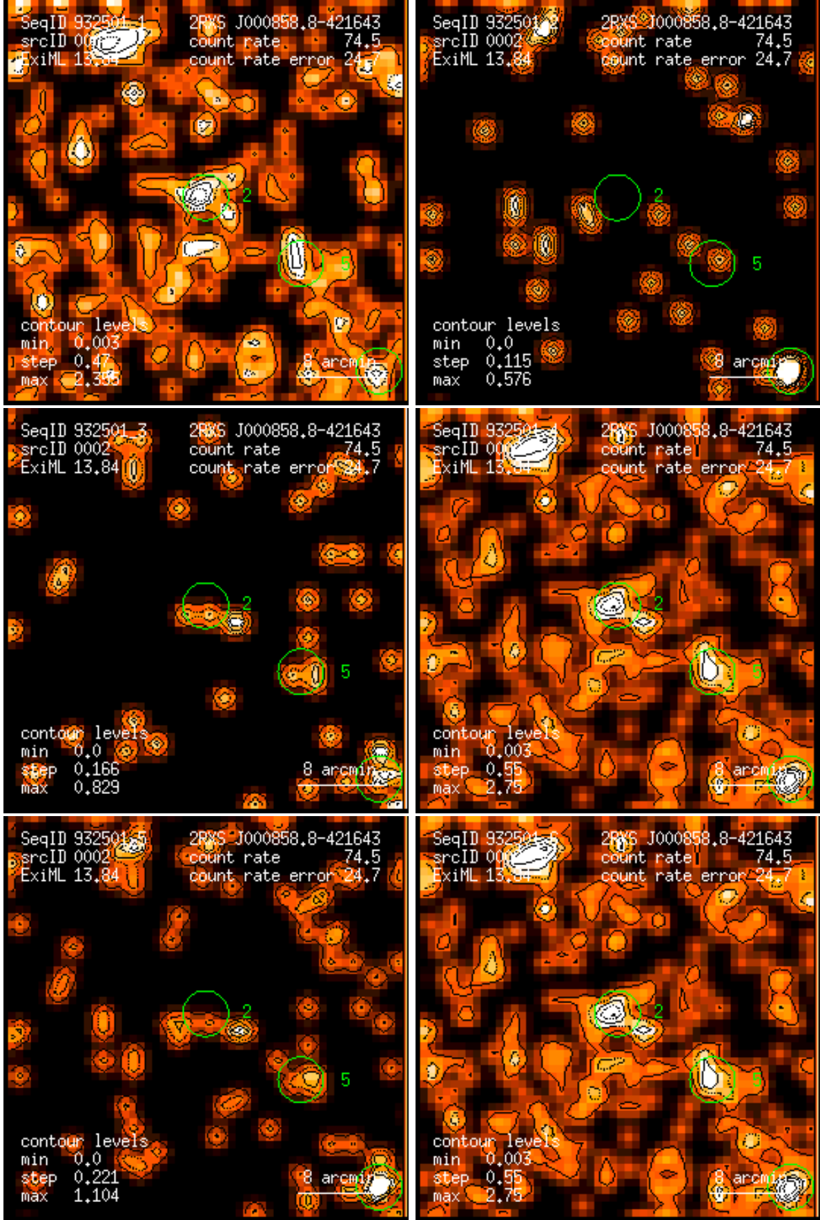
Figure 2: RASS 932501: detection 0002: band rate images, Gaussian filter: (1) PSPC channels 11 – 41, (2) 52 – 90, (3) 91 – 201, (4) 11 – 235, (5) 52 – 201, (6) 11 – 201. Broad band rates in counts/ks. Band rate contour levels in counts/ks/arcmin 2 .
