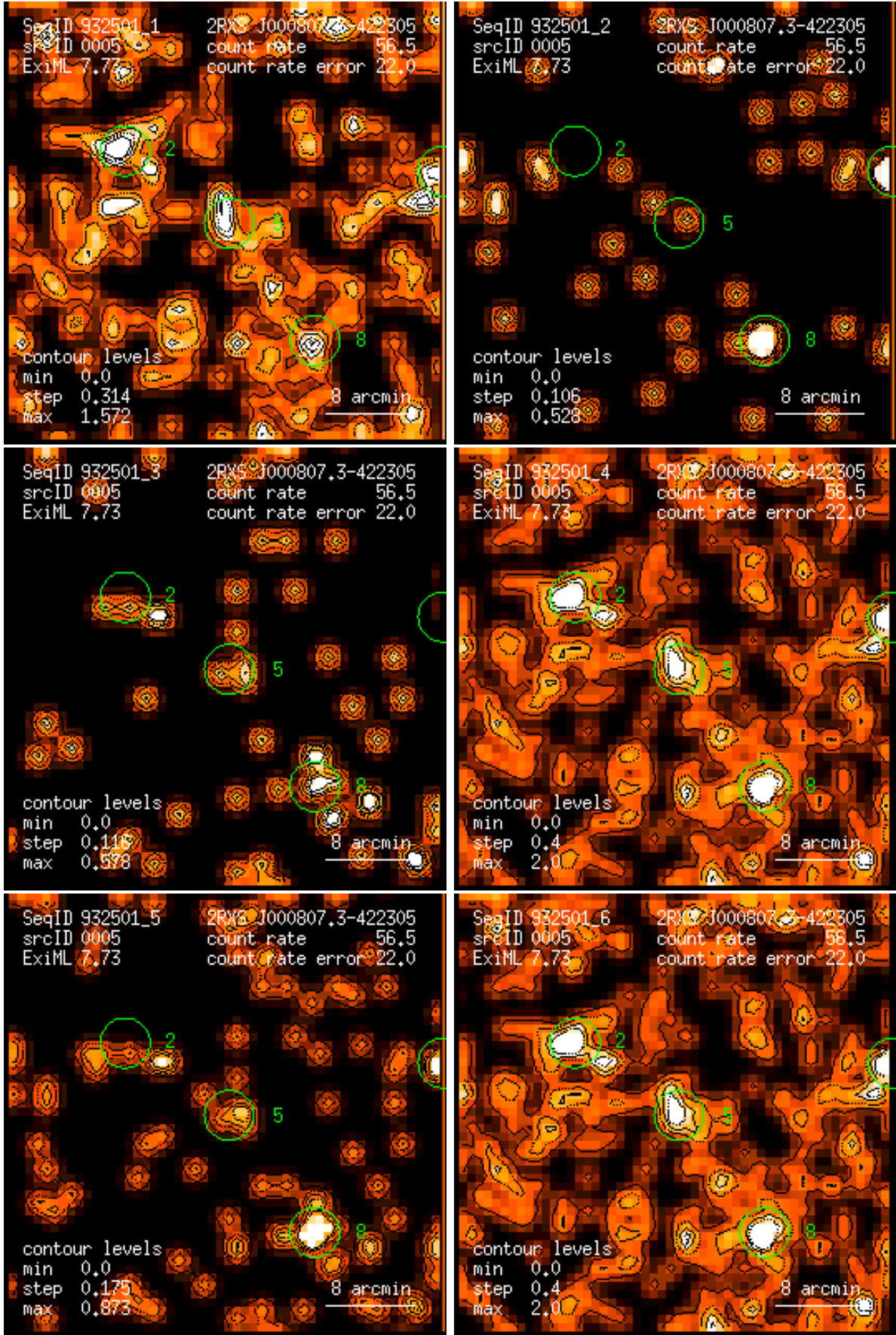
Figure 5: RASS 932501: detection 0005: band rate images, Gaussian filter: (1) PSPC channels 11 – 41, (2) 52 – 90, (3) 91 – 201, (4) 11 – 235, (5) 52 – 201, (6) 11 – 201. Broad band rates in counts/ks. Band rate contour levels in counts/ks/arcmin 2 .
