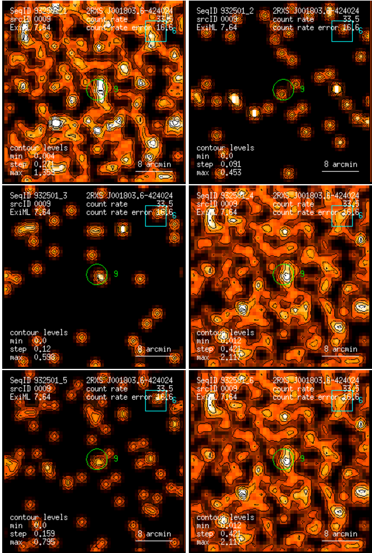
Figure 9: RASS 932501: detection 0009: band rate images, Gaussian filter: (1) PSPC channels 11 – 41, (2) 52 – 90, (3) 91 – 201, (4) 11 – 235, (5) 52 – 201, (6) 11 – 201. Broad band rates in counts/ks. Band rate contour levels in counts/ks/arcmin 2 .
